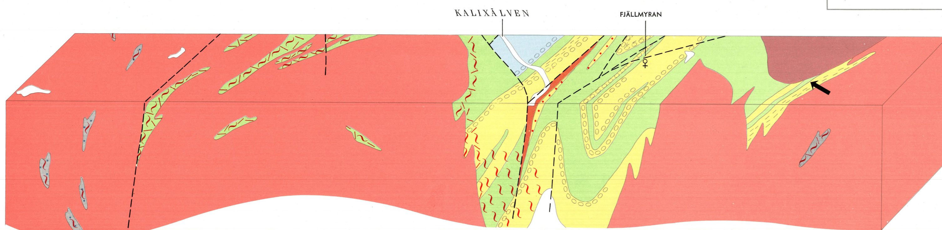
Blockdiagram IV
