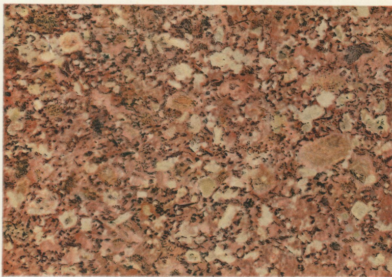
2 GRANITE-PORPHYRY. Elfdalen, Dalarna.
