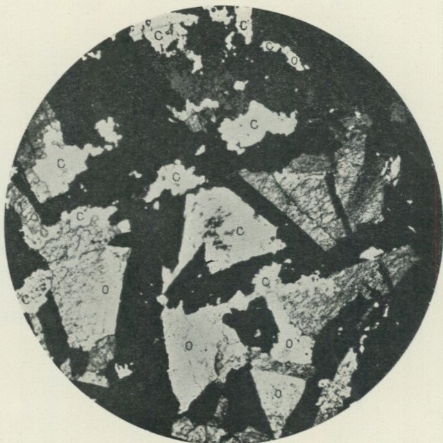
Fig. 2. Microphoto. of cerium ore from Bastnäs, rich in orthite; ord. light, magn. 13 times. Dark areas and light areas marked O are orthite (note twinning), light areas marked C are cerite.
