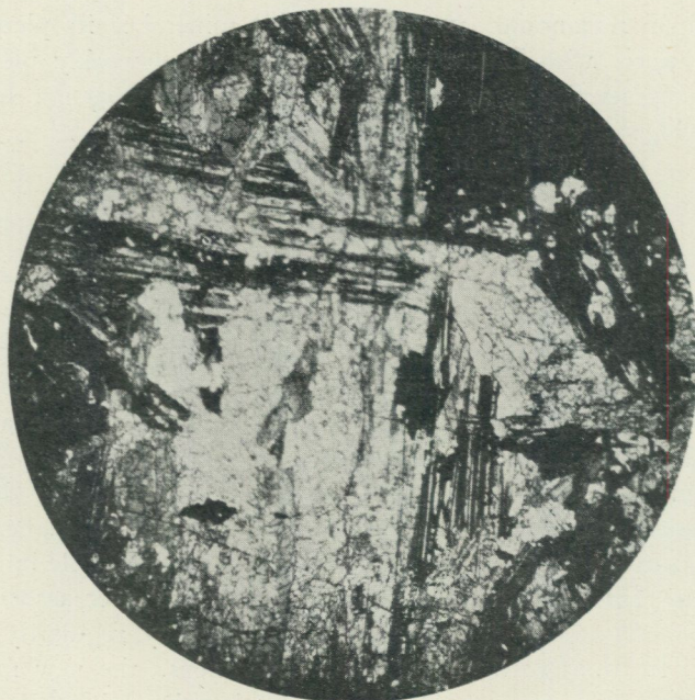
Fig. 3. Microphoto. of cerium ore from Bastnäs, showing intergrowths of orthite and törnebohmite; ord. light, magn. 10 times. The orthite is mostly dark, the törnebohmite white.
