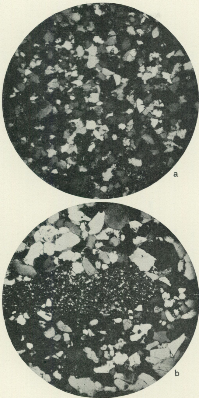
Fig. 3 a, b. Light-grey, fine-grained sandstone with the bulk of the quartz grains angular; in b, a fragment of greenish-grey clay shale; microphoto., nic. crossed, \times 60 . Mossberga; a, level 47.2 m; b, level 47.3 m.
