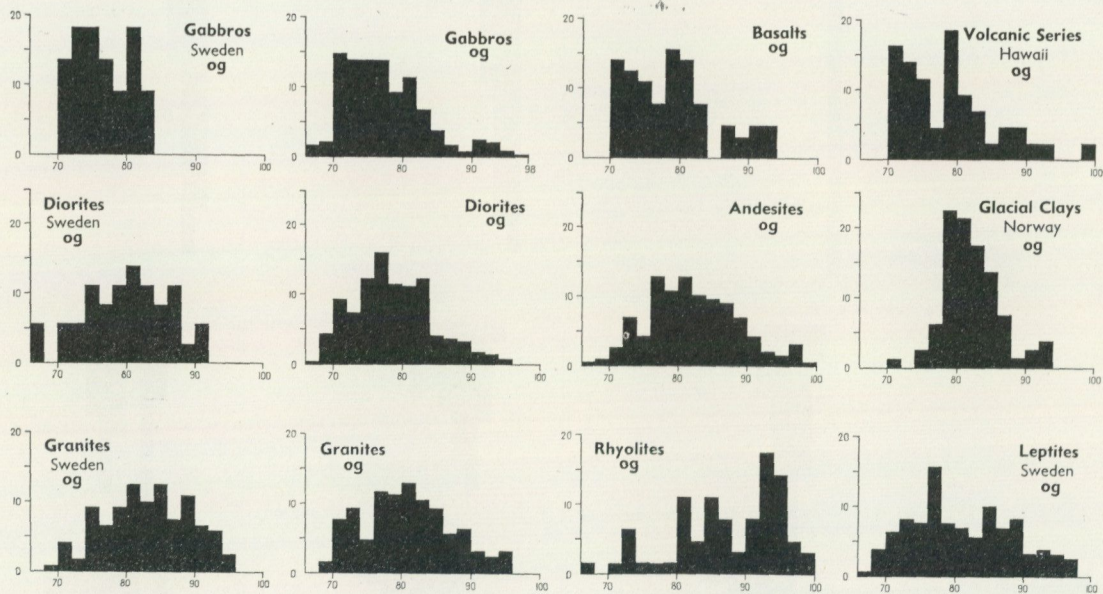
Fig. 3. Histograms of the percentage frequency distribution (ordinate) of the degree of oxidation (abscissa) in the igneous rocks and glacial clay.
