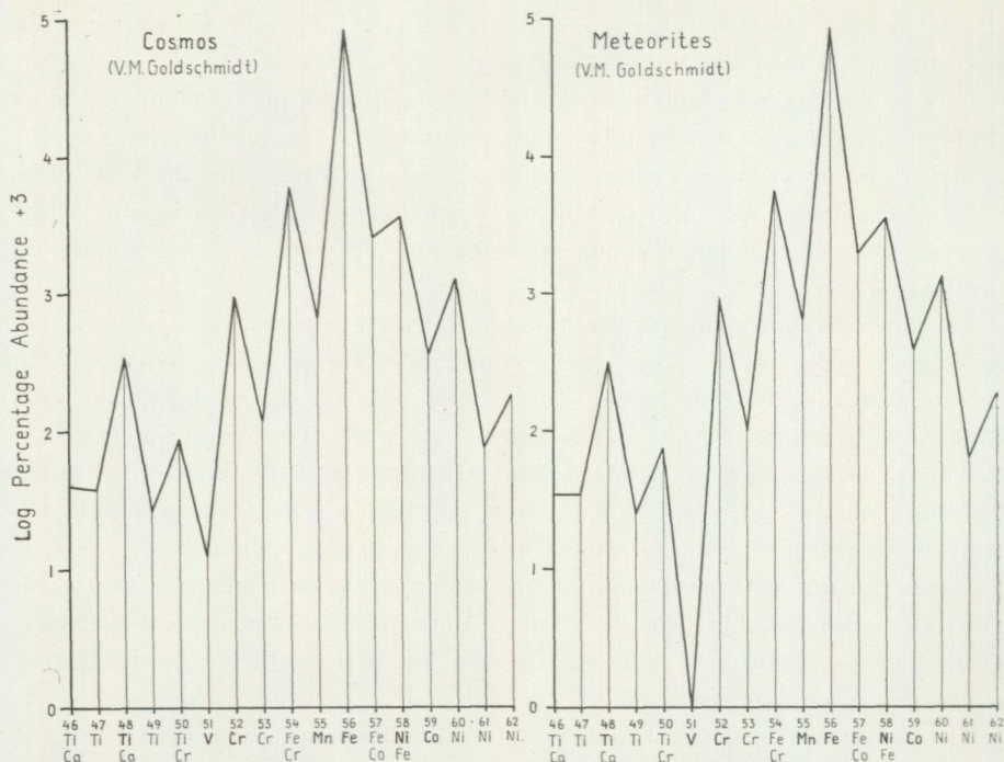
Fig. 19. Diagram of the percentage abundance of the ferride isotopes with mass-numbers 46—62 in Cosmos and Meteorites (mean).
