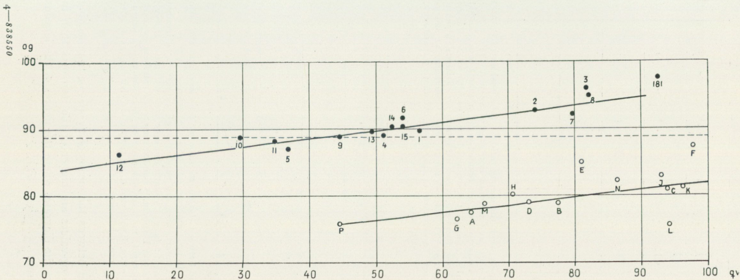
Fig. 16. Diagram of the relationship between the quartz ratio qv (abscissa) and the degree of oxidation og (ordinate). The upper curve: pre-Cambrian iron ores of Sweden. The lower curve: the igneous rocks and glacial clay.
