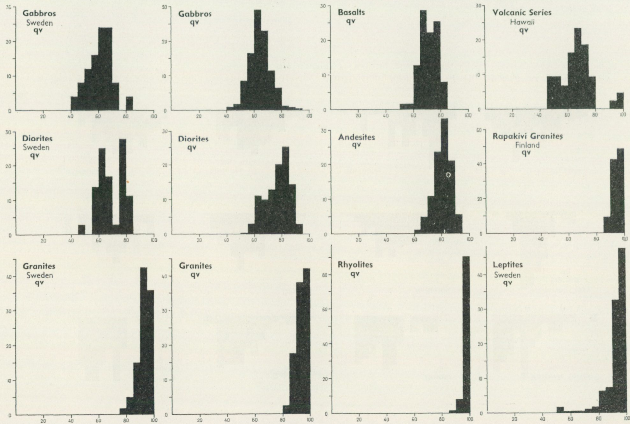
Fig. 2. Histograms of the percentage frequency distribution (ordinate) of the quartz ratio q_v (abscissa) in the igneous rocks.
