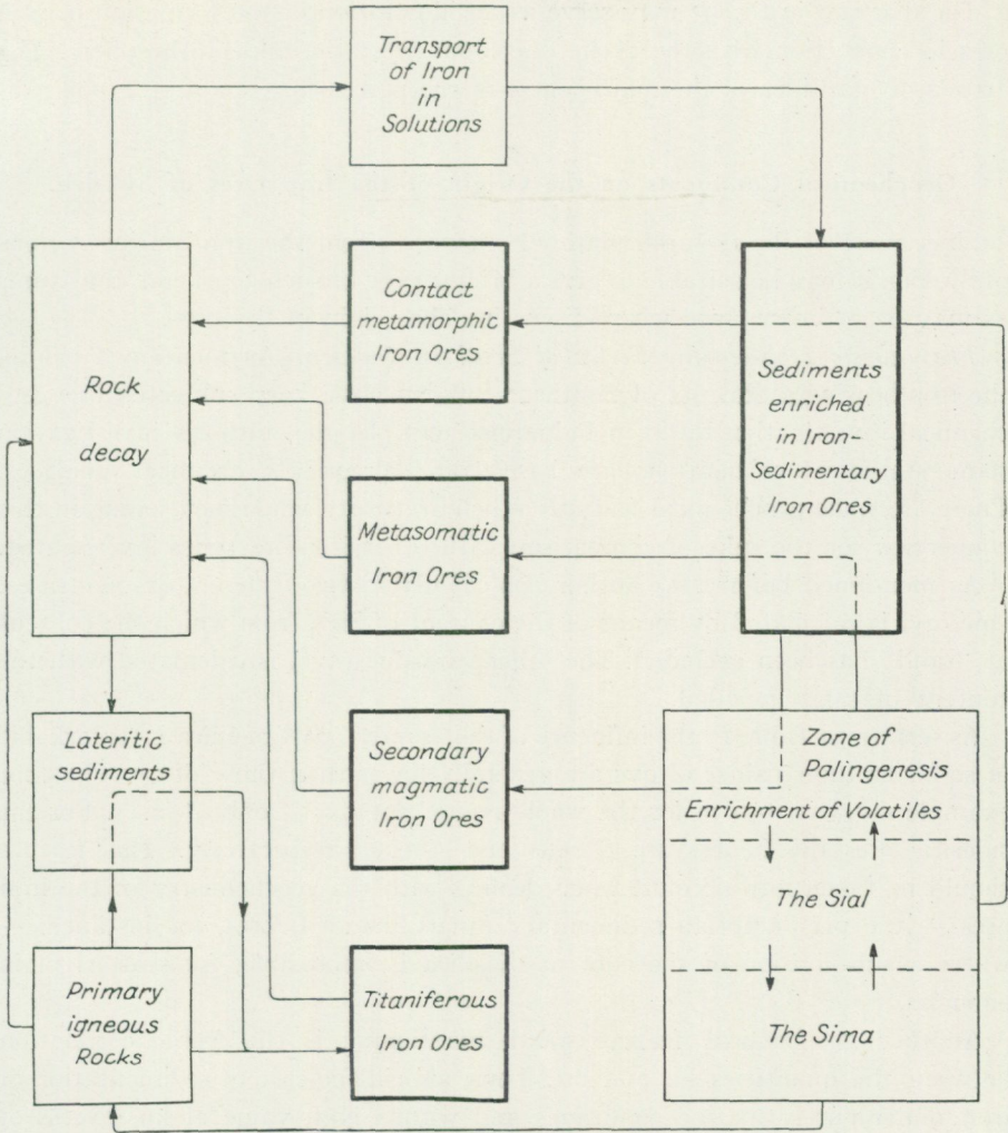
Fig. 31. Diagram illustrating the formation of iron ores in an orogene cycle in the upper lithosphere. The arrows indicate the main course of the processes.
