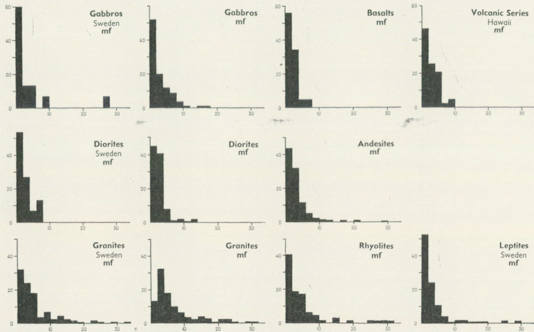
Fig. 7. Histograms of the percentage frequency distribution (ordinate) of the ratio Mn/Fe mf (abscissa) in the igneous rocks.
