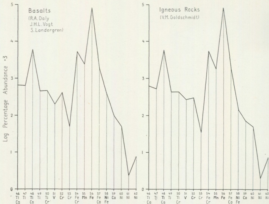
Fig. 21. Diagram of the percentage abundance of the ferride isotopes with mass-numbers 46—62 in basalts and in the igneous rocks (mean).
