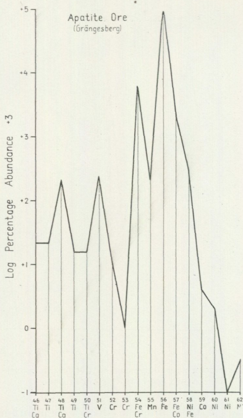
Fig. 24. Diagram of the percentage abundance of the ferride isotopes with mass-numbers 46—62 in apatite iron ores of Grängesberg, Sweden.
