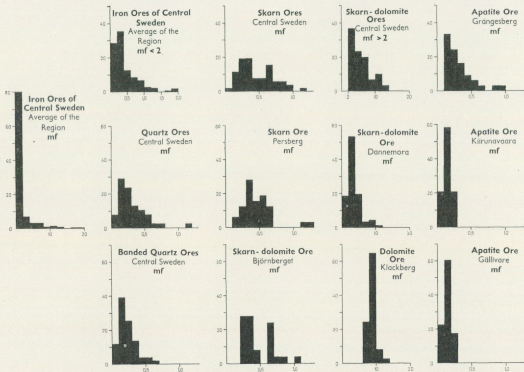
Fig. 11. Histograms of the percentage frequency distribution (ordinate) of the ratio Mn/Fe mf (abscissa) in some Swedish iron ore types.
