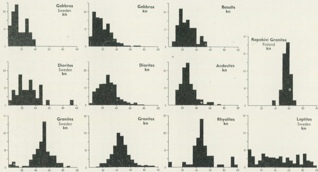
Fig. 6. Histograms of the percentage frequency distribution (ordinate) of the ratio K_2O/Na_2O kn (abscissa) in the igneous rocks.
