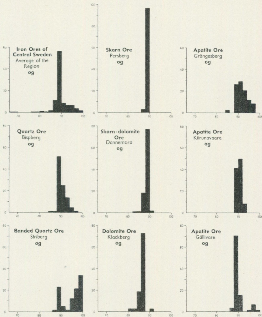
Fig. 9. Histograms of the percentage frequency distribution (ordinate) of the degree of oxidation og (abscissa) in some Swedish iron ore types.
