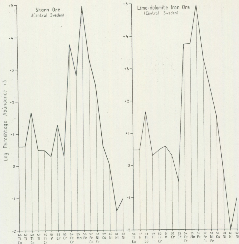
Fig. 27. Diagram of the percentage abundance of the ferride isotopes with mass-numbers 46—62 in skarn and lime-dolomite ores from central Sweden.
