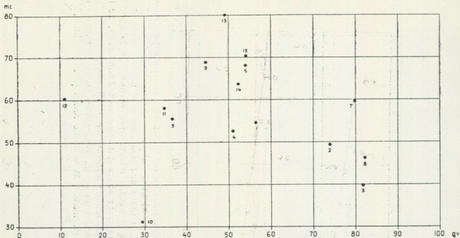
Fig. 17. Diagram of the relationship between the quartz ratio qv (abscissa) and the ratio MgO/CaO mc (ordinate) in pre-Cambrian iron ores of Sweden.
