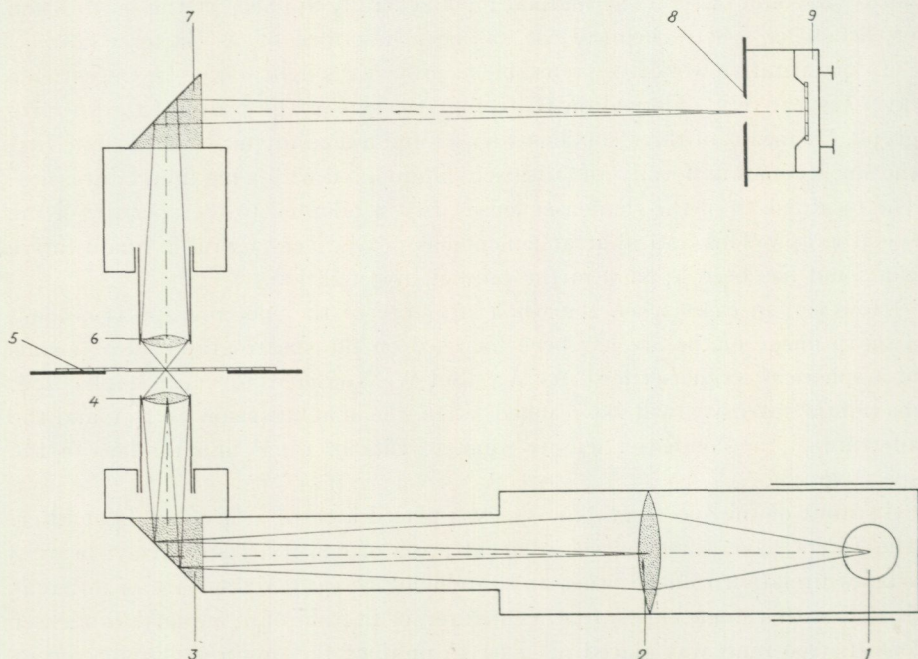
Fig. 1. The optic arrangement in the Stålex spectrophotometer. 1 light source, 2, 4 and 6 condenser lenses, 3 and 7 glass-prisms and mirrors, 5 table with the spectral plate, 8 slit, and 9 photoelectric cell.
