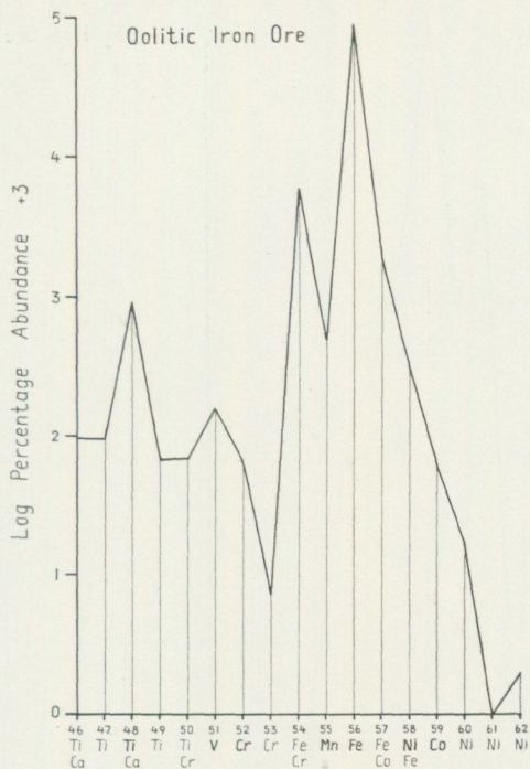
Fig. 25. Diagram of the percentage abundance of the ferride isotopes with mass-numbers 46—62 in oolitic iron ores.
