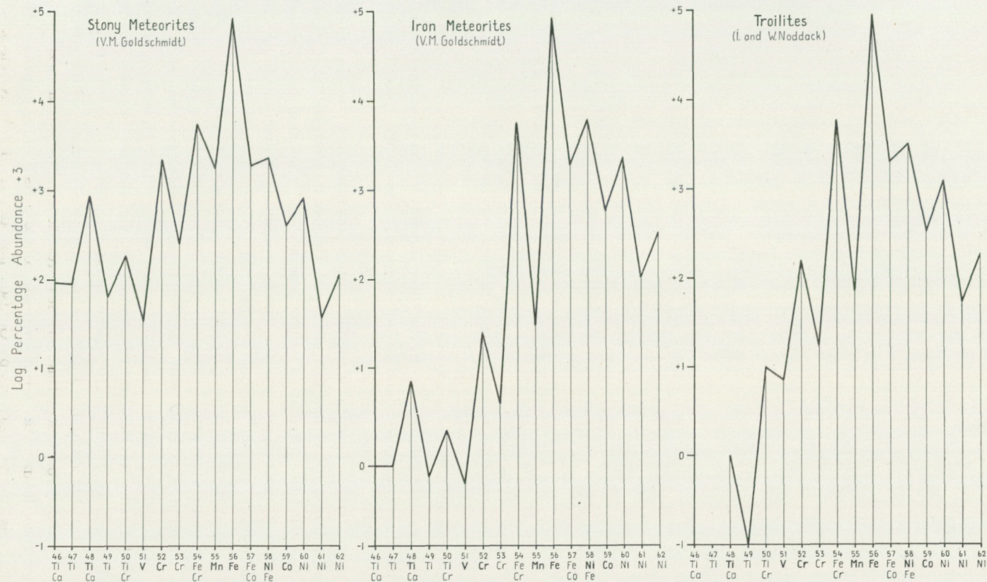
Fig. 20. Diagram of the percentage abundance of the ferrides isotopes with mass-numbers 46—62 in the three meteoritic phases.
