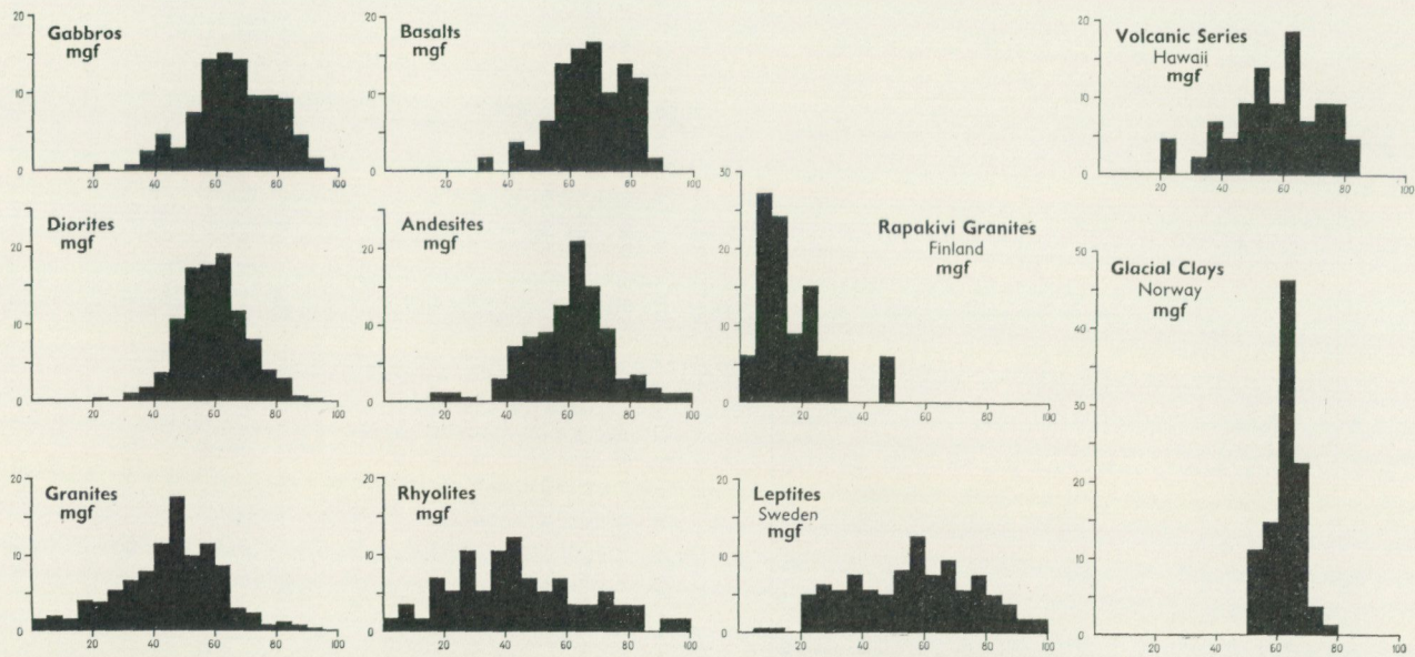
Fig. 5. Histograms of the percentage frequency distribution (ordinate) of the ratio MgO/FeO mgf (abscissa) in the igneous rocks and glacial clay.
