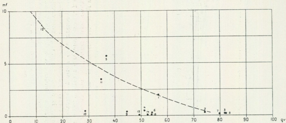
Fig. 18. Diagram of the relationship between the quartz ratio qv (abscissa) and the ratio Mn/Fe mf (ordinate) in pre-Cambrian iron ores of Sweden.
