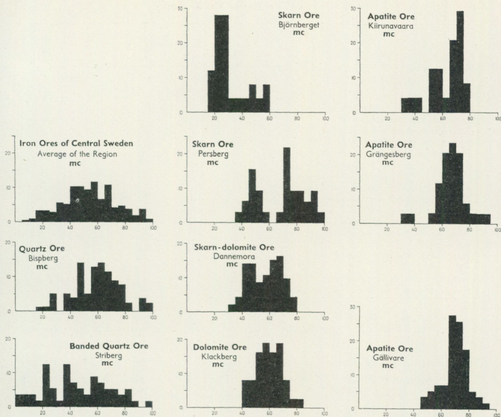
Fig. 10. Histograms of the percentage frequency distribution (ordinate) of the ratio MgO/CaO mc in some Swedish iron ore types.
