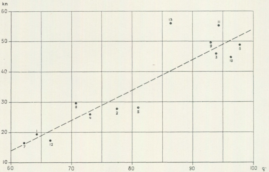
Fig. 15. Diagram of the relationship between the quartz ratio qv (abscissa) and the ratio K_2O/Na_2O kn (ordinate) in the igneous rocks and glacial clay.
