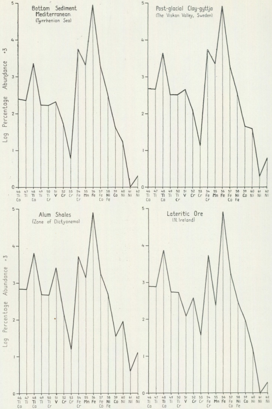
Fig. 22. Diagram of the percentage abundance of the ferride isotopes with mass-numbers 46—62 bottom sediment from the Tyrrhenian Sea (Mediterranean), post-glacial clay-gyttja from the Viskan valley, Sweden, alum shale, Sweden, and lateritic sediment, N. Ireland.
