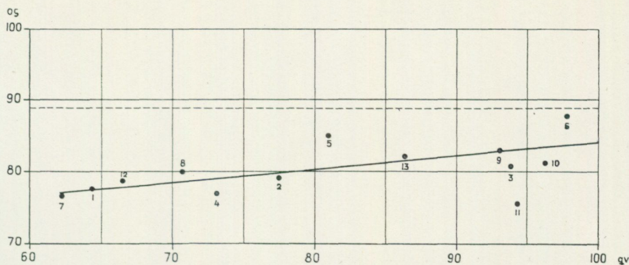
Fig. 12. Diagram of the relationship between the quartz ratio qv (abscissa) and the degree of oxidation og (ordinate) in the igneous rocks and glacial clay.
