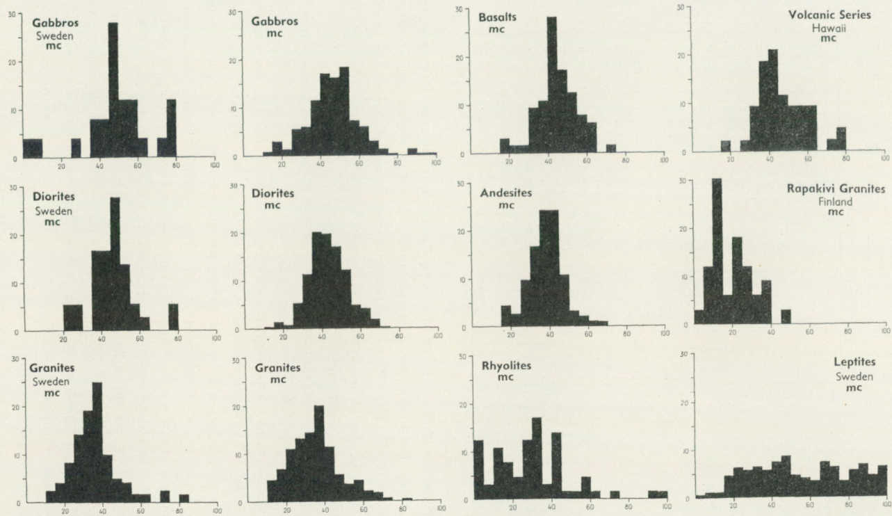
Fig. 4. Histograms of the percentage frequency distribution (ordinate) of the ratio MgO/CaO mc (abscissa) in the igneous rocks.
