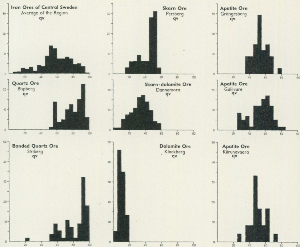
Fig. 8. Histograms of the percentage frequency distribution (ordinate) of the quartz ratio q_v (abscissa) in some Swedish iron ore types.
