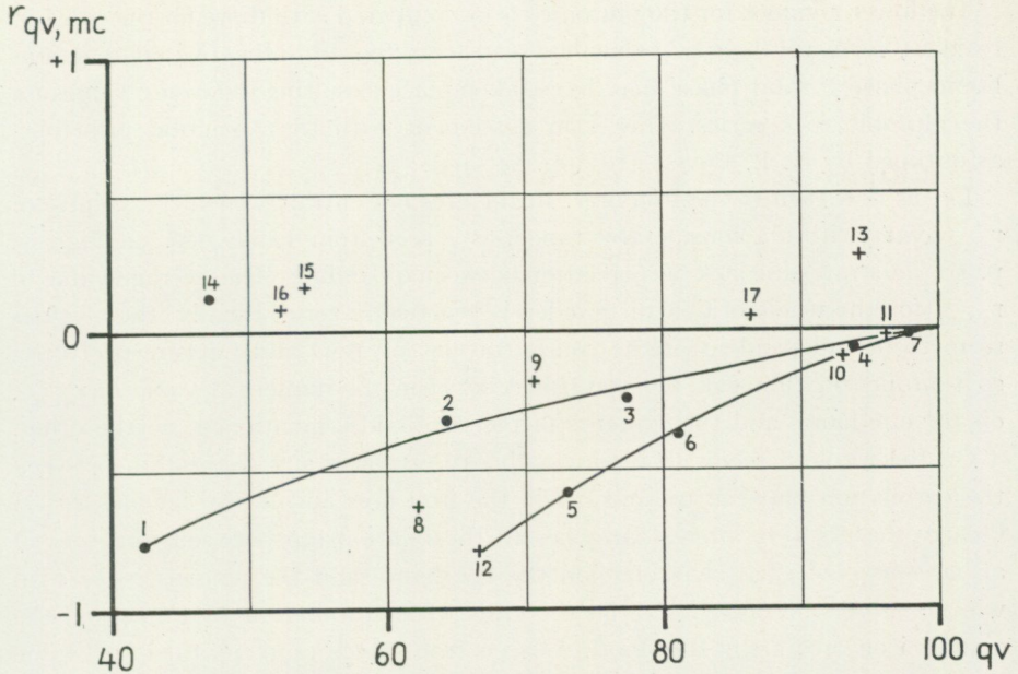
Fig. 30. Diagram and curves showing the decreasing value for r_{qv,mc} as the quartz ratio ( qv ) increases in the igneous rocks. The r -values for the titaniferous iron ores, the apatite iron ores, and the glacial clay are plotted in the diagram.
