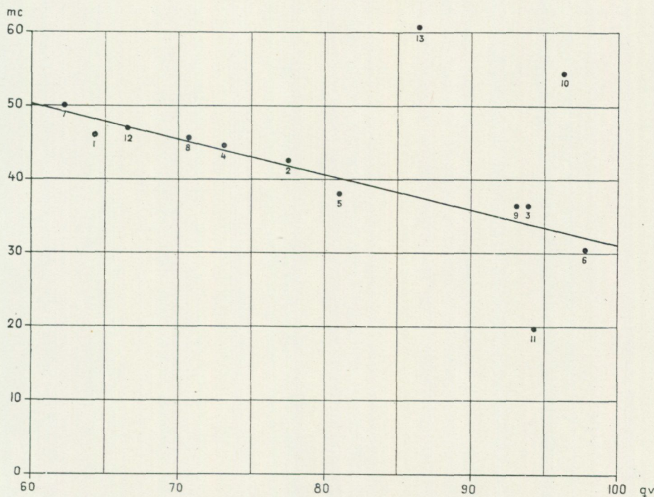
Fig. 13. Diagram of the relationship between the quartz ratio qv (abscissa) and the ratio MgO/CaO mc (ordinate) in the igneous rocks and glacial clay.
