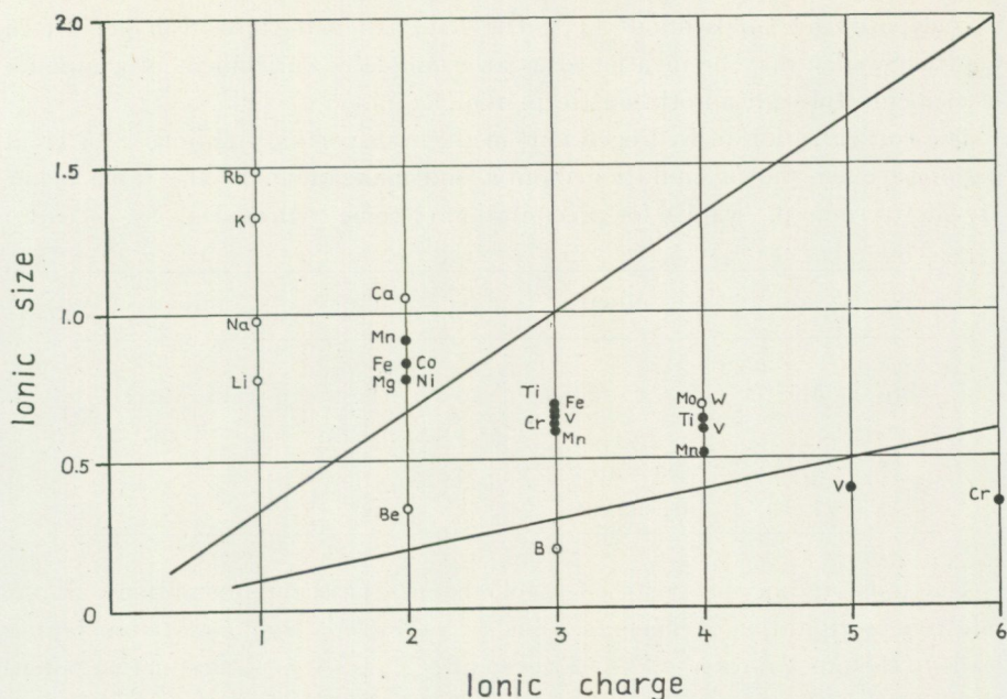
Fig. 29. Diagram of the distribution of elements in solution. (After V. M. Goldschmidt.) Filled circles are ferrides.
