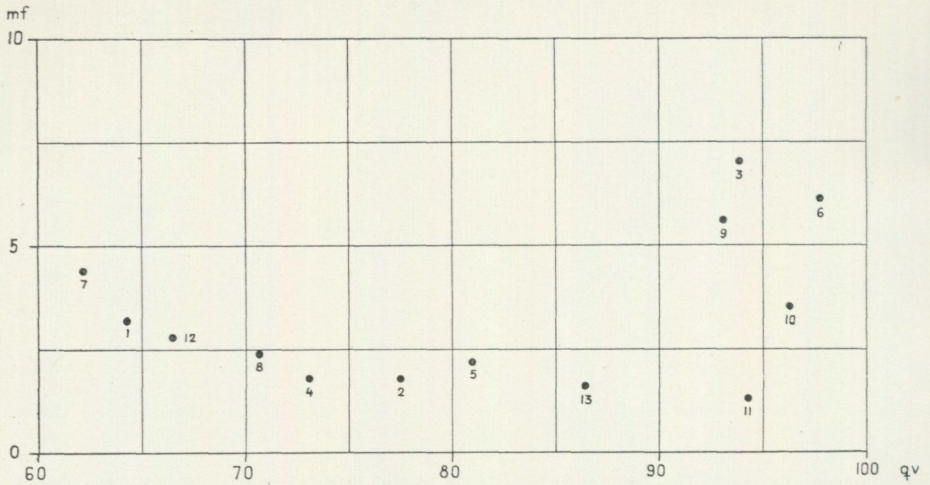
Fig. 14. Diagram of the relationship between the quartz ratio qv (abscissa) and the ratio Mn/Fe mf (ordinate) in the igneous rocks and glacial clay.
