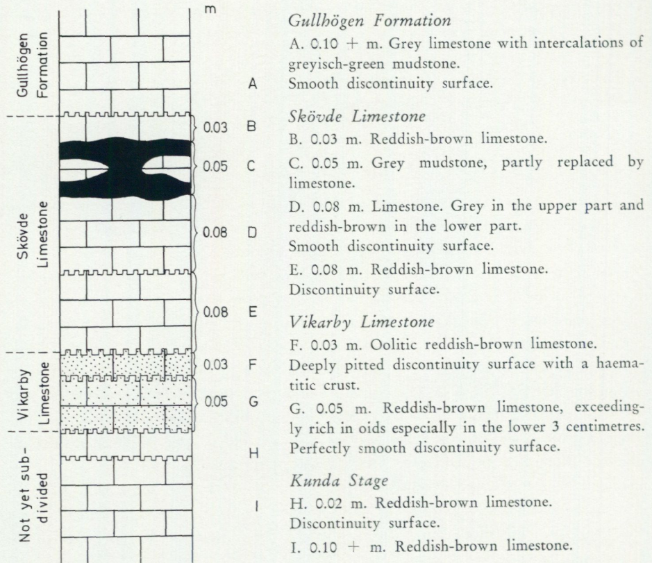
Fig. 1. Section through the Lower Viruan and the topmost Oelandian beds at the Gullhögen quarry.
