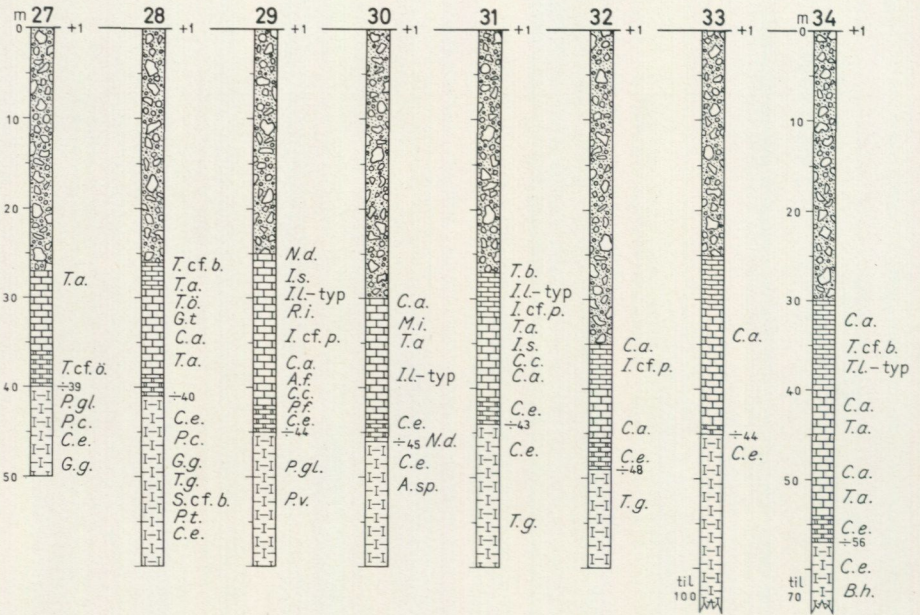
Fig. 4. Profiler af borerne 27-34. Columnar sections of wells nos. 27-34.
