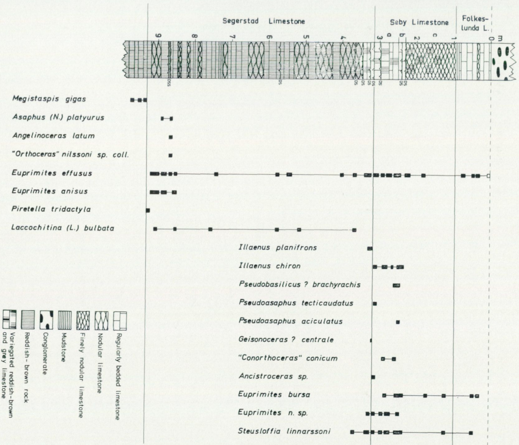
Fig. 4. Range of selected species in the Gtigas , Segerstad, Seby and Folkelslunda Limestones of the Lunne section. DS: discontinuity surface, DSS: double discontinuity surfaces.
