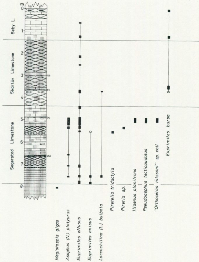
Fig. 19. Range of selected species in the Gigas , Segerstad, Skärlov and Seby Limestones of the Oppbodarna section. For legend, see Fig. 4.
