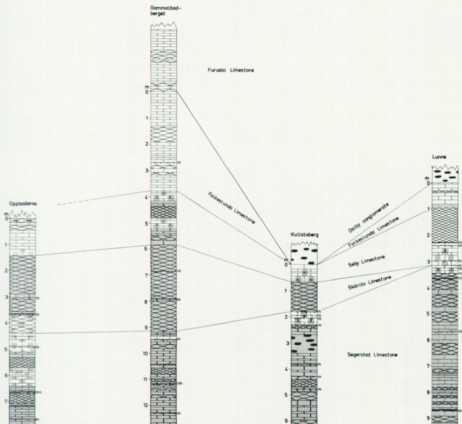
Fig. 21. A comparison of the Aserian, Lasnamägian and Uhakuan sections in the Åsarne, Lockne and Brunflo areas. For legend, see Fig. 4.
