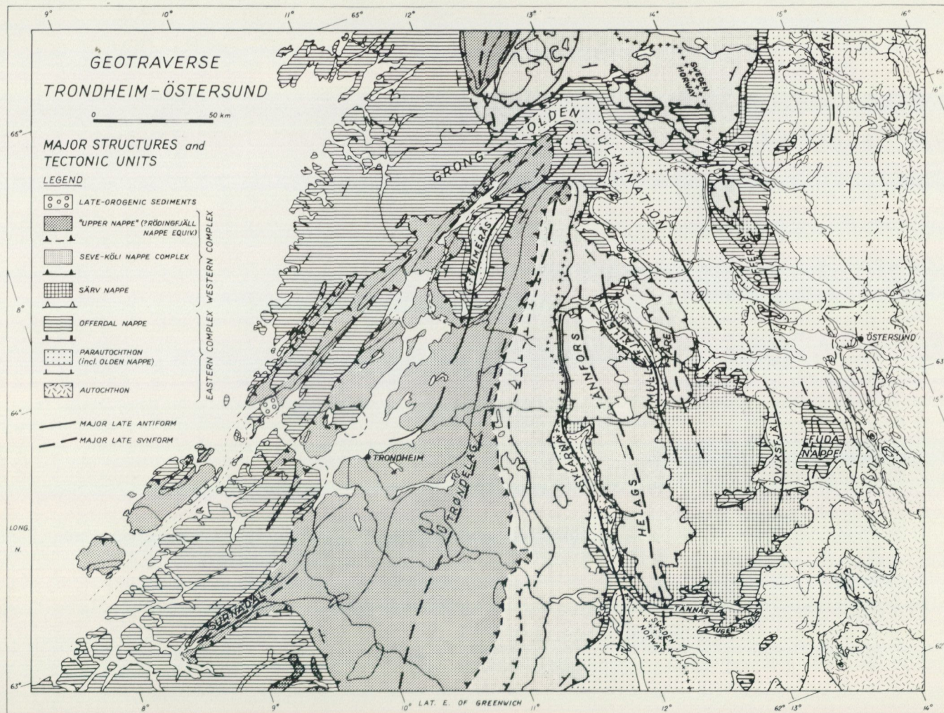
Fig. 2. General tectonic units and structures.
