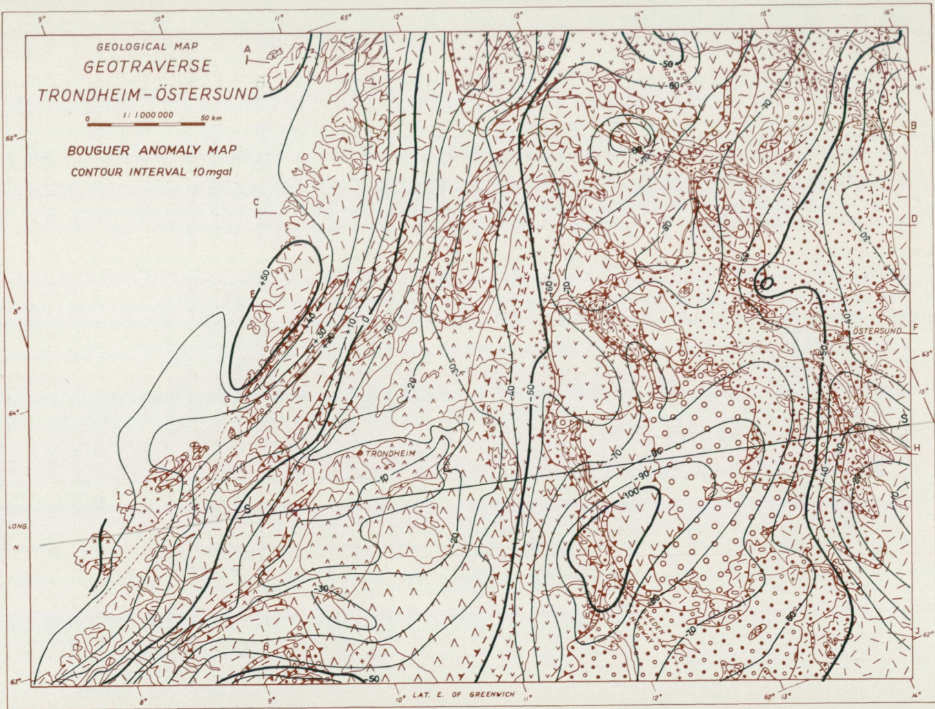
Fig. 10. Bouguer Anomalies over the Geotransverse area. Compilation based on Wieland (1951), Grønlie and Ramberg (1970) and Kaneström and Haugland (1971). The line S-S marks the location of the deep seismic profile (Vogel and Lund 1972).
