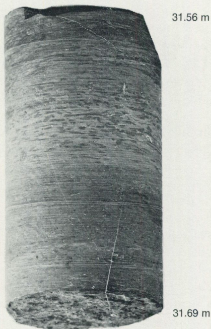
Fig. 3. Core section between 31.69–31.56 m showing speckled shale. Diplograptus multidentis Zone. Diameter of core 7 cm.
