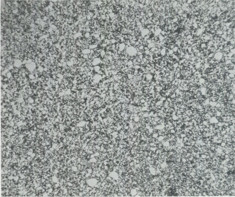
Fig. 4. Quartz grains between 17.83 and 17.803 m of the core. Thin section 8 ×.
