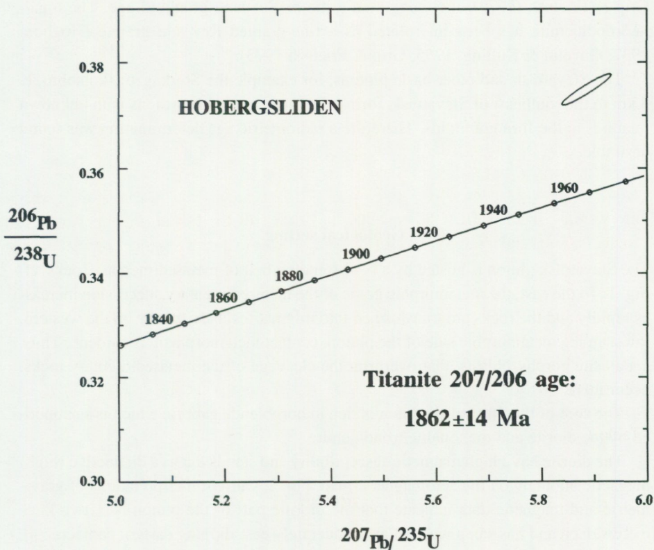
Fig. 3. Concordia plot for the Hobergsliden titanite.
