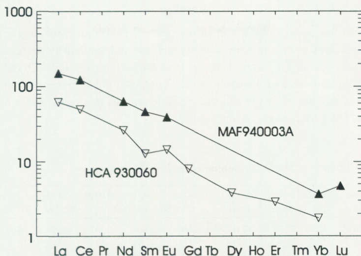
Fig. 4. REE plot for the Stavaträsk diorite and tonalite/trondhjemite. Normalization according to Sun (1982).
