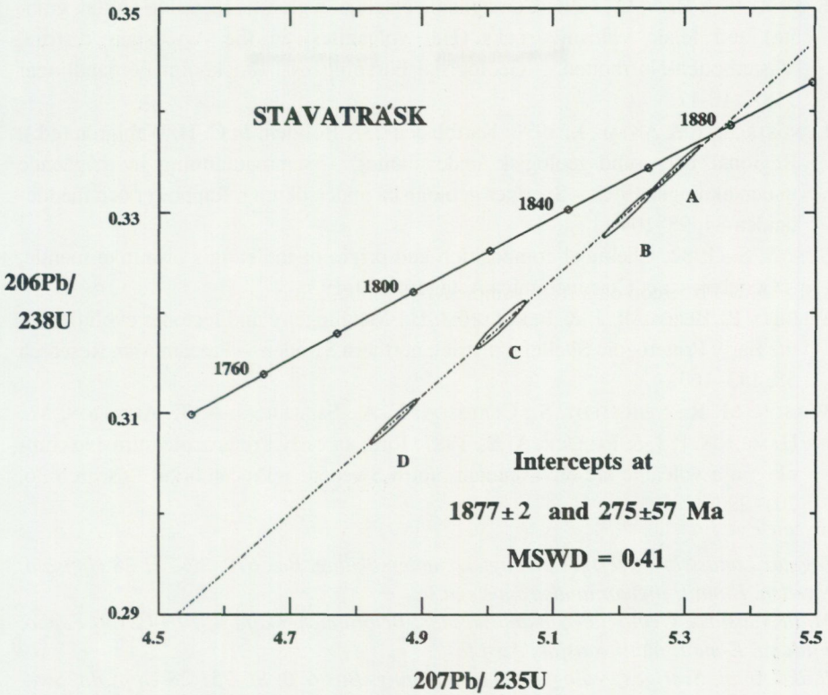
Fig. 5. Concordia plot for the zircons of the Stavatråsk diorite.
