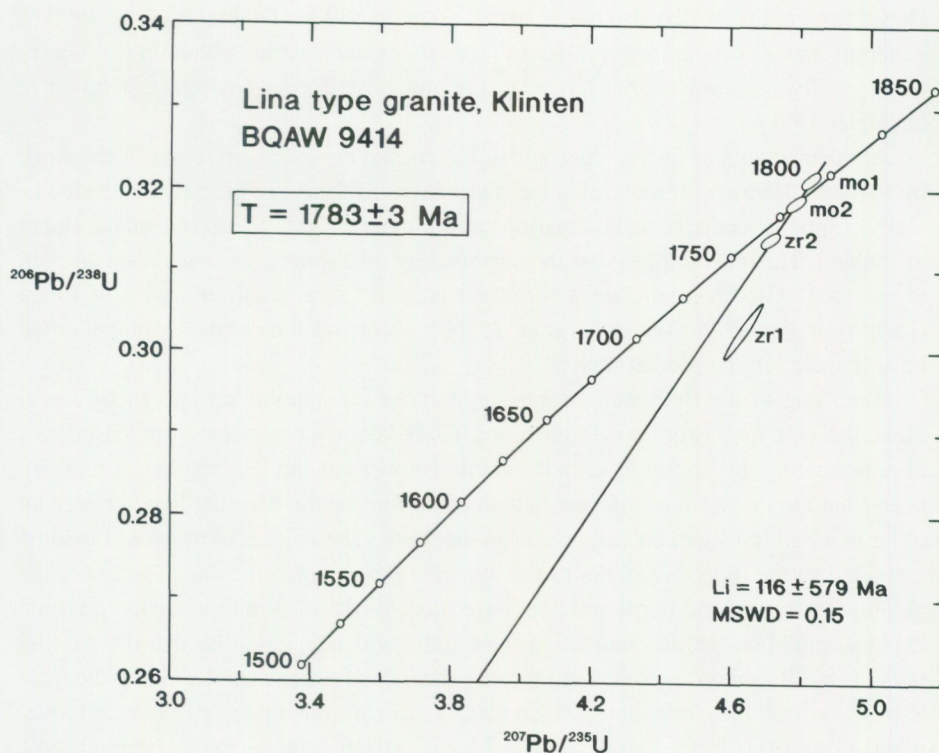
Fig. 2. U-Pb concordia diagram for zircons and monazites from the Klinten sample.
