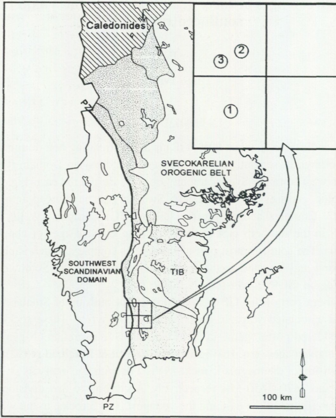
Fig. 1. Simplified map of southern Sweden showing the major Precambrian units. Stippled area represents the Transscandinavian Igneous Belt (TIB). Location of the four map-sheets Väjö (NV, SV, NO and SO) and the investigated samples 1, MHW 94060, 2, MHW 94606 and 3, MHW 94613, are indicated.
