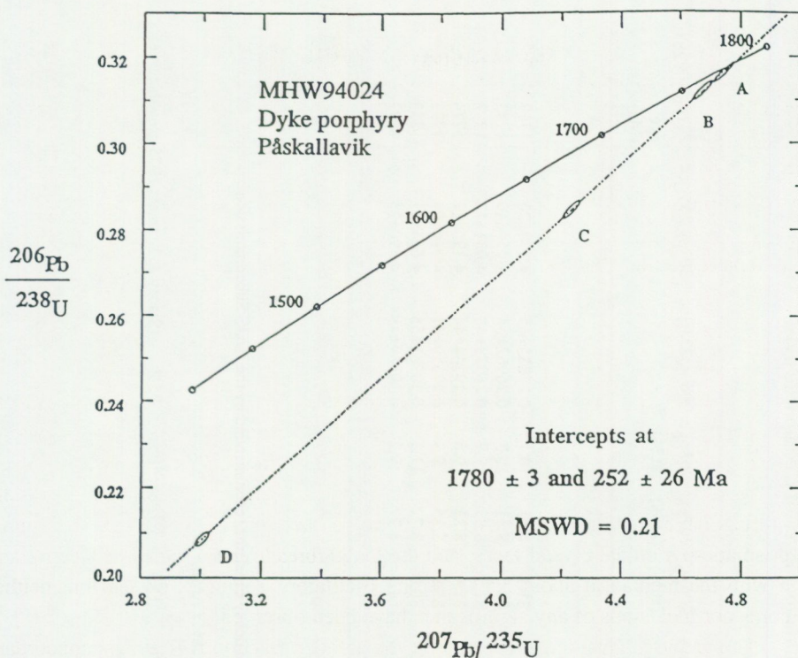
Fig. 2. U-Pb concordia diagram for zircons from sample MHW 94024, reddish grey dyke porphyry, Paskallavik porphyry.
