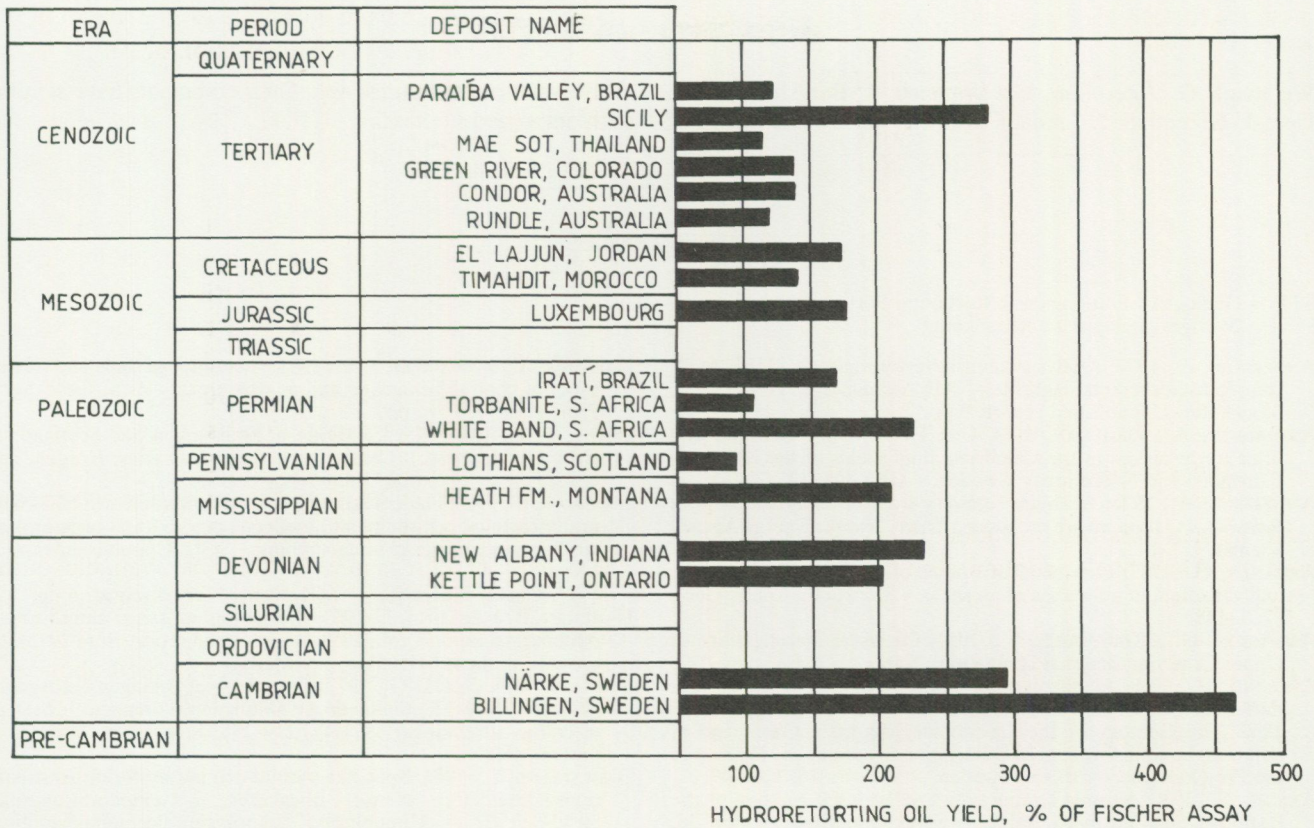
Fig. 24. Hydroretorting assay test results (from Janka & Rex 1984). The Närke and Billingen samples (Fischer assays of 4.4% and 1.5%, respectively) yielded 134 litres/tonne and 73 litres/tonne oil, respectively, when retorted in an atmosphere of hydrogen under pressure (7 MPa).
