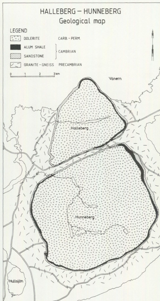
Fig. 11 Bedrock geology of the Halleberg-Hunneberg outlier (from Sidenbladh 1870).
