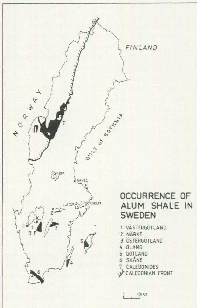
Fig. 3. Alum shale occurrences in Sweden (B-F = Billingen-Falbygden, H = Hallberg-Hunneberg, K = Kinnekulle).
