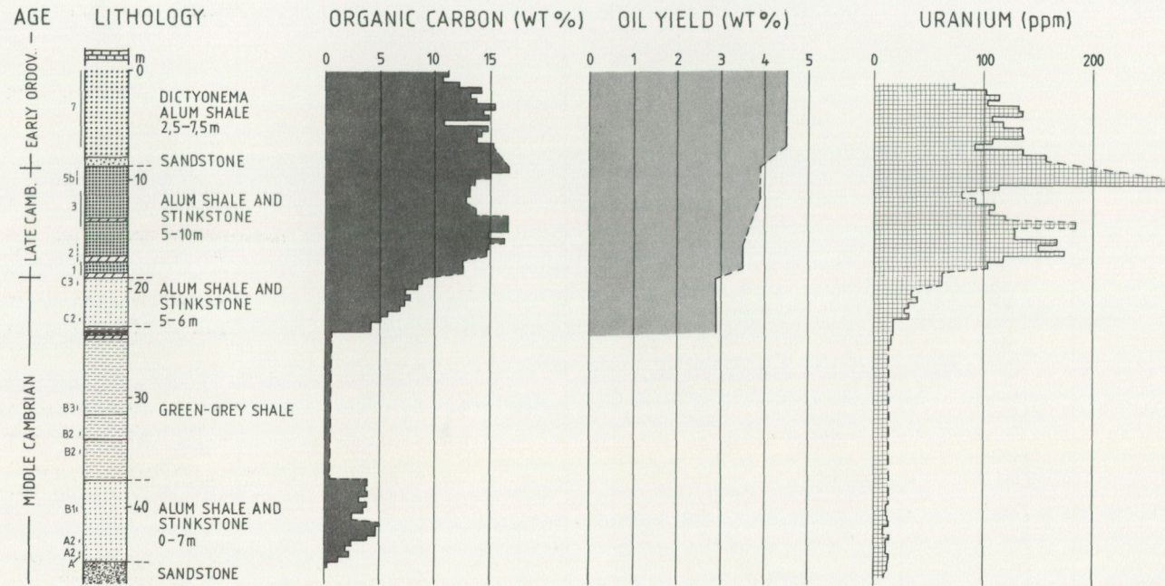
Fig. A4. The alum shales in the Östergötland outlier are illustrated by data from the Näsja drillhole (Wikman et al. 1982). Chemical data are taken from Dahlman (1962, unpublished report). The thicknesses cited are relevant for the outlier in general. Note that the alum shale facies in the early Middle Cambrian is restricted to western areas.
