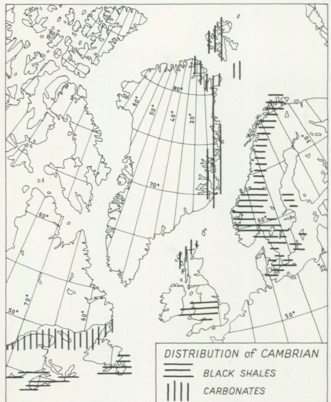
Fig. 22. Late Palaeozoic reconstruction of the Caledonian-Appalachian orogen showing the distribution of the Cambrian black shale and limestone facies (from Gee et al. 1974).
