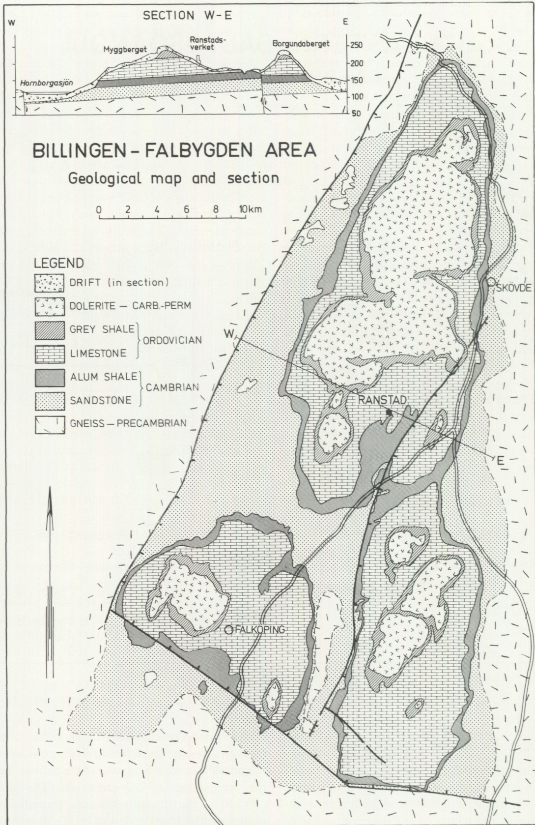
Fig. 5 Bedrock geology of the Billingen-Falbygden outlier, Västergötland.
