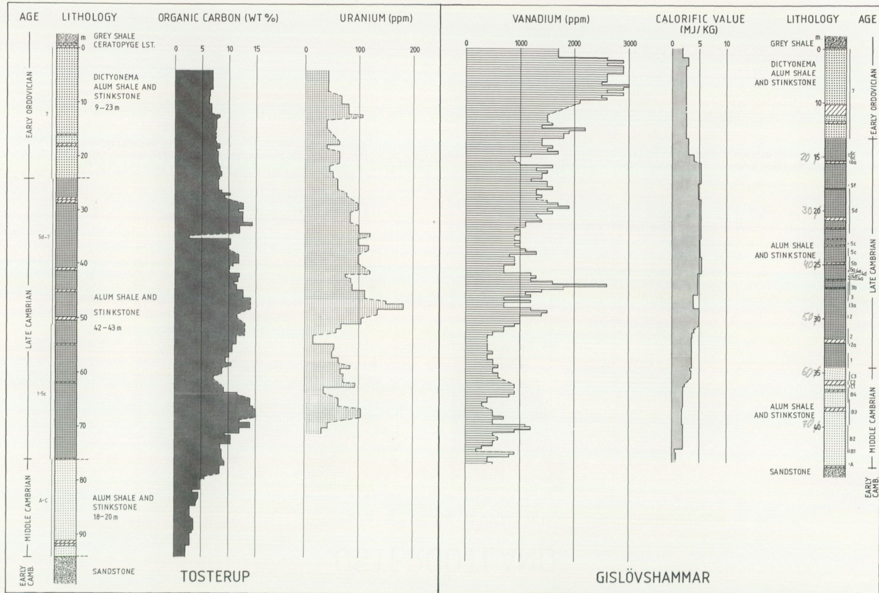
Fig. A5. The alum shales in Skåne are illustrated by data from two drillholes, located at Tosterup (Dahlman 1962, unpublished report) and Gislövshammar (Westergård, 1944a). Analyses of C_{org} were obtained from SGU's archives. The thicknesses cited are representative for southeastern areas. The development of the alum shales inferred to be present beneath the thicker Ordovician and younger strata is unknown.
