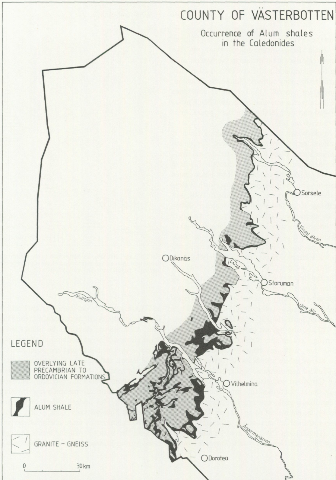
Fig. 21. Distribution of the alum shales in western Västerbotten County. The formation occurs in the autochthonous sedimentary rocks of the Caledonian Front, in the lower nappes and in the parautochthonous and lower allochthonous cover strata in the windows. Areas are also marked where the alum shales are covered by Ordovician strata or thrust sheets of Upper Proterozoic and Lower Cambrian sandstones and quartzites. The alum shales probably also occur at greater depths beneath the higher nappes (based on a compilation for Radonutredningen 1979 by T. Thelander, Ds Jo 1979:9, Appendix 2:2).
