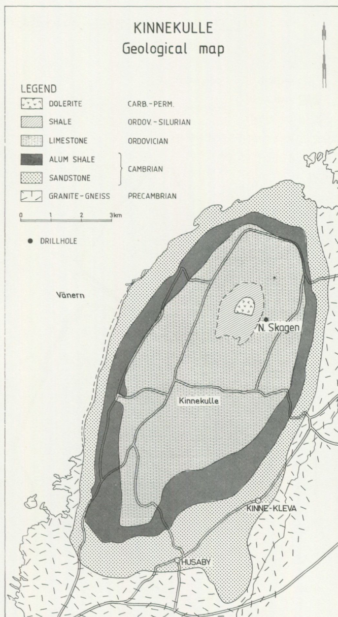
Fig. 10. Bedrock geology of the Kinneulle outlier (from Westergård 1943).
