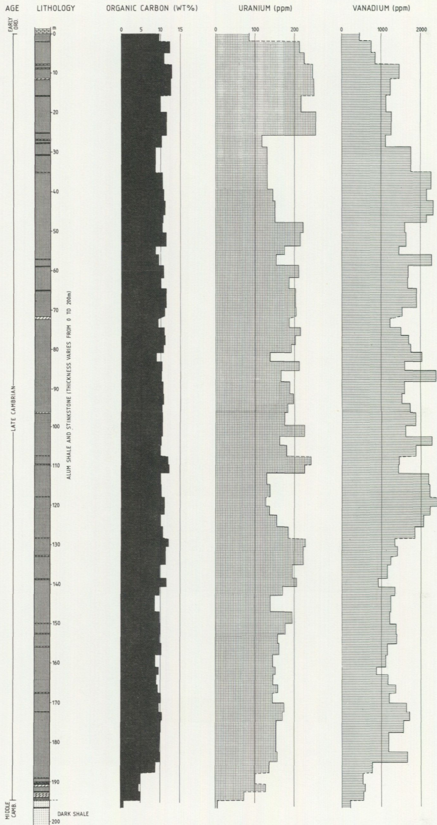
Fig. A7. The alum shales in Jämtland are illustrated by data from the Myrviken 78005 drillhole (Gee et al. 1982, unpublished report) located near Myrviken in the Southern Storsjön Area. The hole was drilled near the crest of the Myrviken Antiform (see Fig. 19, section E-F) and contains one of the greatest thicknesses of black shales in Jämtland.
