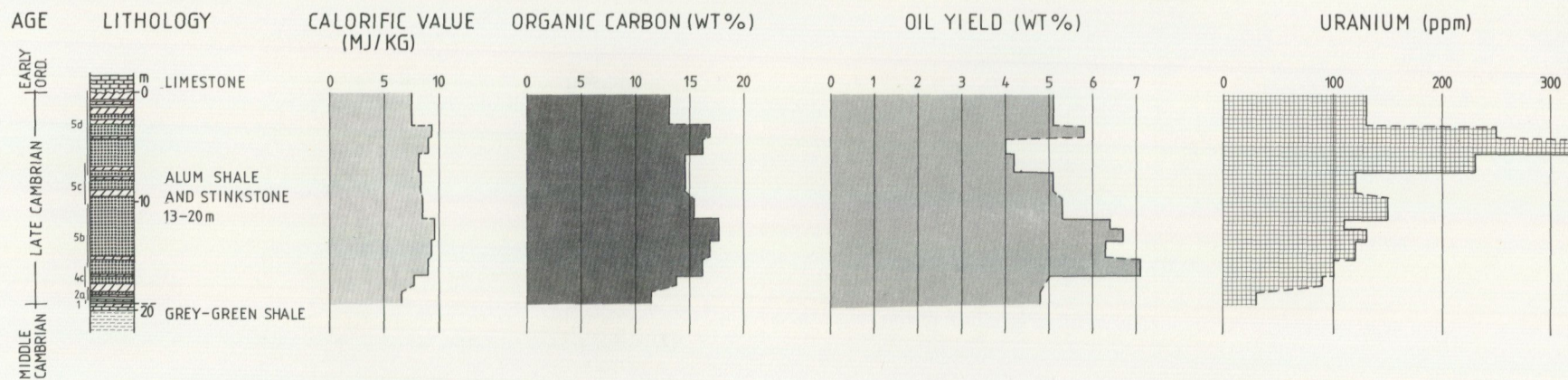
Fig. A3. The alum shales in the Närke outliers are illustrated by data from a Hynneberg drillhole (Eklund in Eklund et al. 1961). Eklund reported the organic content as wt % kerogen. To simplify comparison with other areas, the kerogen values have been converted to wt % C_{org} on the basis of kerogen analyses provided in Assarsson & Grundulis (1961). The high uranium peak (>300 ppm) in the Peltura scarabaeoides zone is probably due to the presence of a kolm lens. The thicknesses cited are representative for both East and West Närke.
