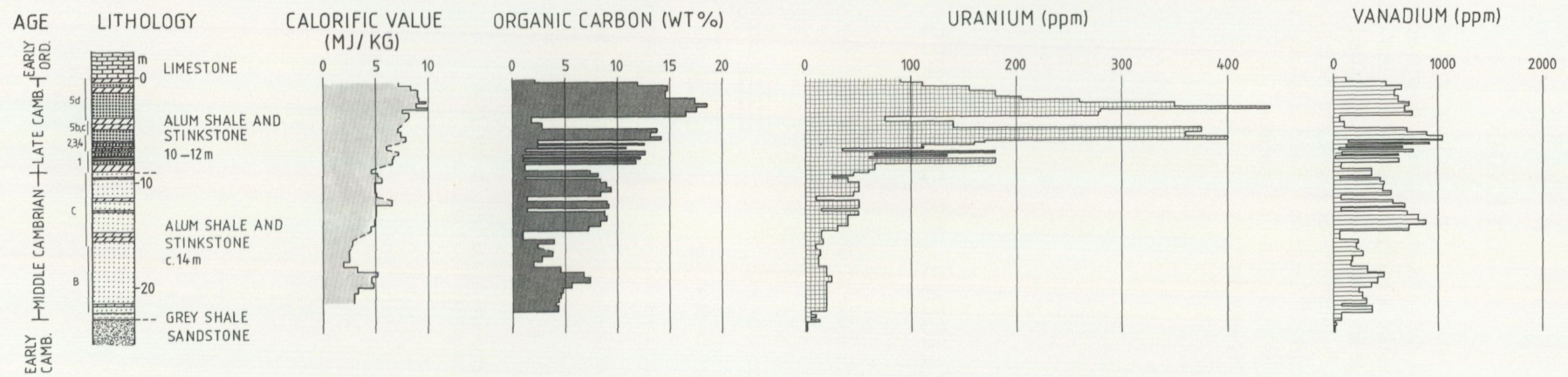
Fig. A1. The alum shales in the Billingen-Falbygden outlier are illustrated by data from drillhole Dbh 65/77 at Ranstad (Andersson 1977, unpublished report). The thicknesses cited are relevant for the outlier in general. Note, however, that the stinkstone in the most uranium-rich section is unusually thick. For biostratigraphical data given to the left of the lithological column see Fig. 2 in the text.
