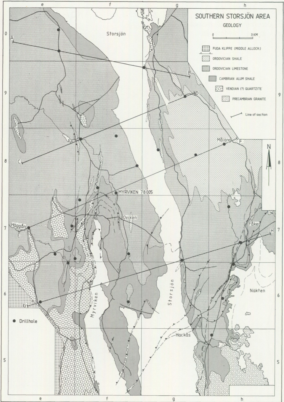
Fig. 18. Bedrock geology of the area of southern Storsjön, Jämtland (based on Gee et al. 1982, unpublished report). The Lines A-B, C-D, E-F and G-H mark the profiles in Fig. 19.
