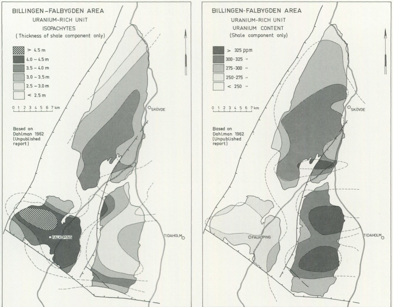
Fig. 8. Relationship between uranium concentration and shale-thickness in the uranium-rich unit of the Ranstad Member of the Alum Shale Formation in the Billingen-Falbygden outlier, Västergötland (from Dahlman & Gee 1977).
