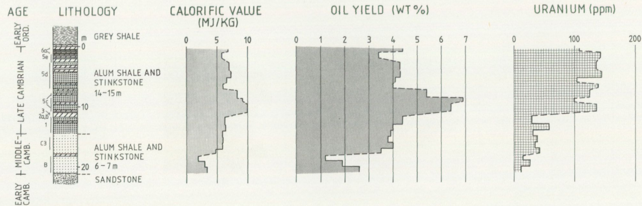
Fig. A2. The alum shales in the Kinnekulle outlier are illustrated by data from drillhole Norra Skagen (Westergård 1943). Analyses of uranium are taken from Dahlman & Eklund 1953 (unpublished report). The thicknesses cited are representative for the entire outlier.
