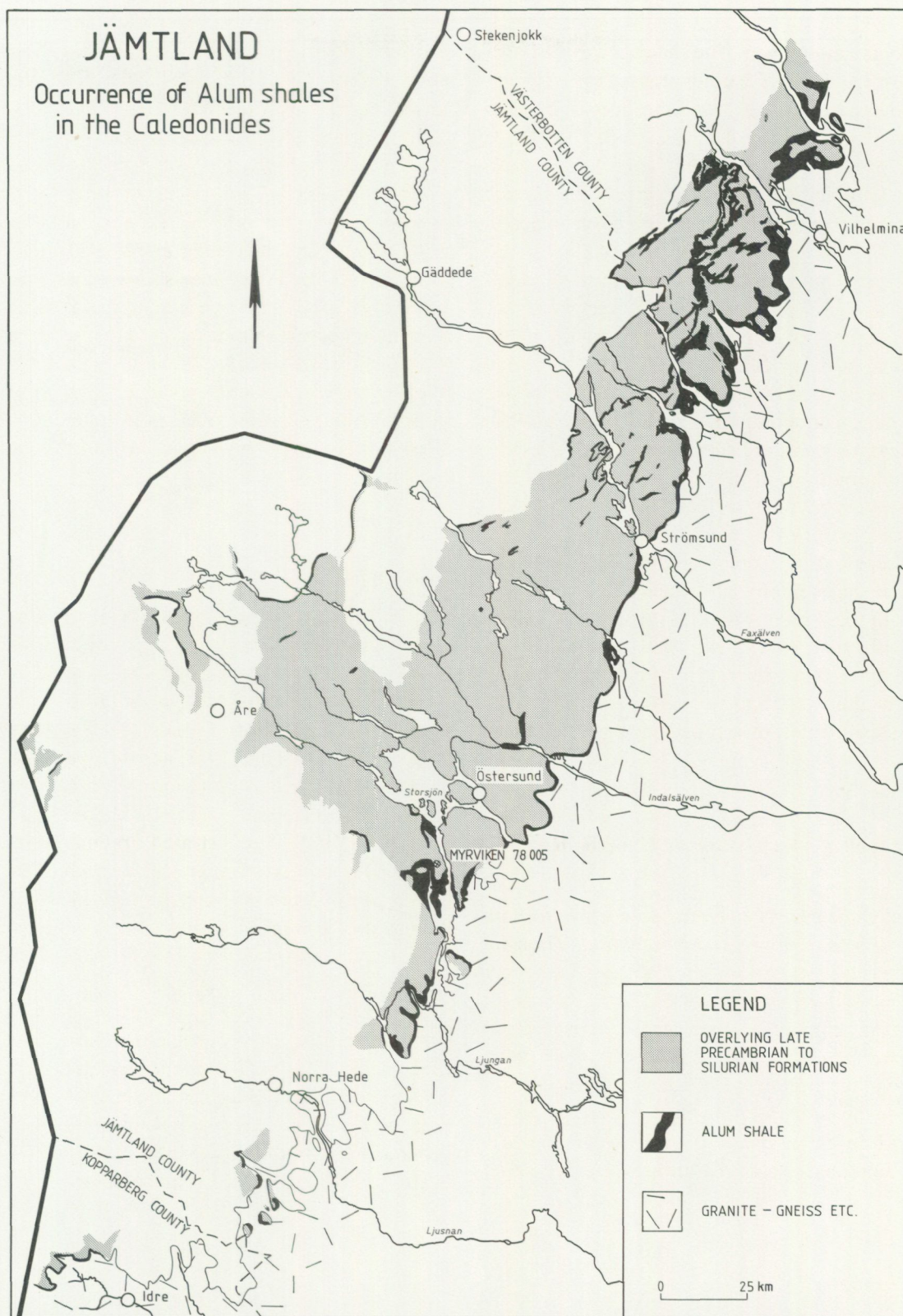
Fig. 17. Distribution of the alum shales in western Jämtland, northernmost Kopparberg and southernmost Västerbotten Counties. Areas are also marked where the alum shales are covered by Ordovician and Silurian strata and/or thrust sheets of Upper Proterozoic/Lower Cambrian sandstones and quartzites. The alum shales probably also occur further west at greater depths beneath the higher nappes (based on a compilation for Radonutredningen 1979 by T. Thelander, Ds Jo 1979:9, Appendix 2:2).
