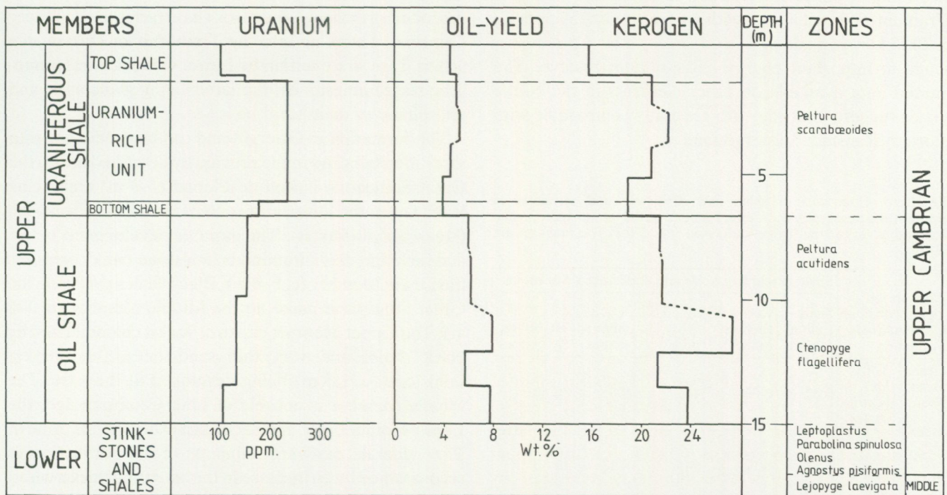
Fig. 13. Variations in the oil yield (Fischer Assay) and contents of uranium and kerogen in the western part of the East Närke outlier (from Andersson et al. 1983). Uranium data are averaged from the Alaborg area (Dahlman 1962, unpublished report), oil yield data derive from the Norrtorp drillcore (Westergård 1941) and kerogen contents have been calculated from the calorific values also provided in Westergård (1941).
