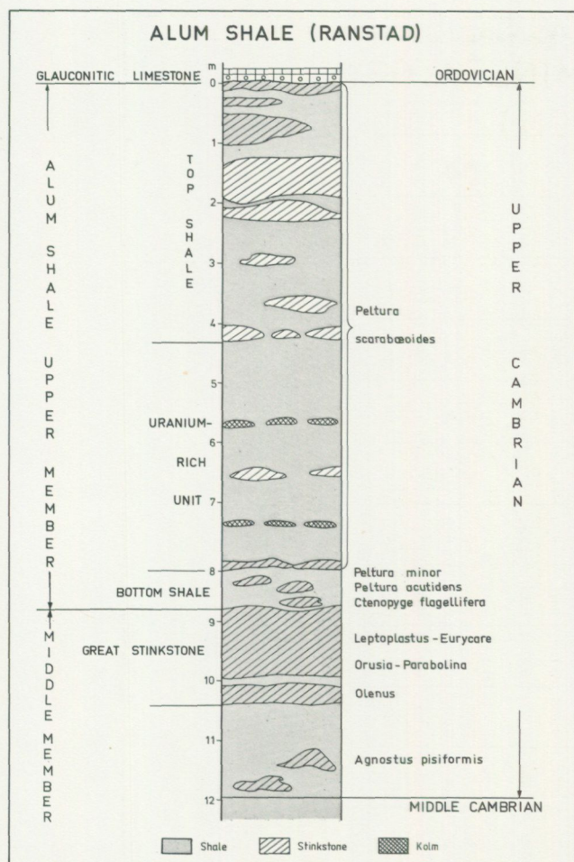
Fig. 7. The Ranstad Member of the Alum Shale Formation in the Ranstad area (from Dahlman & Gee 1977).
