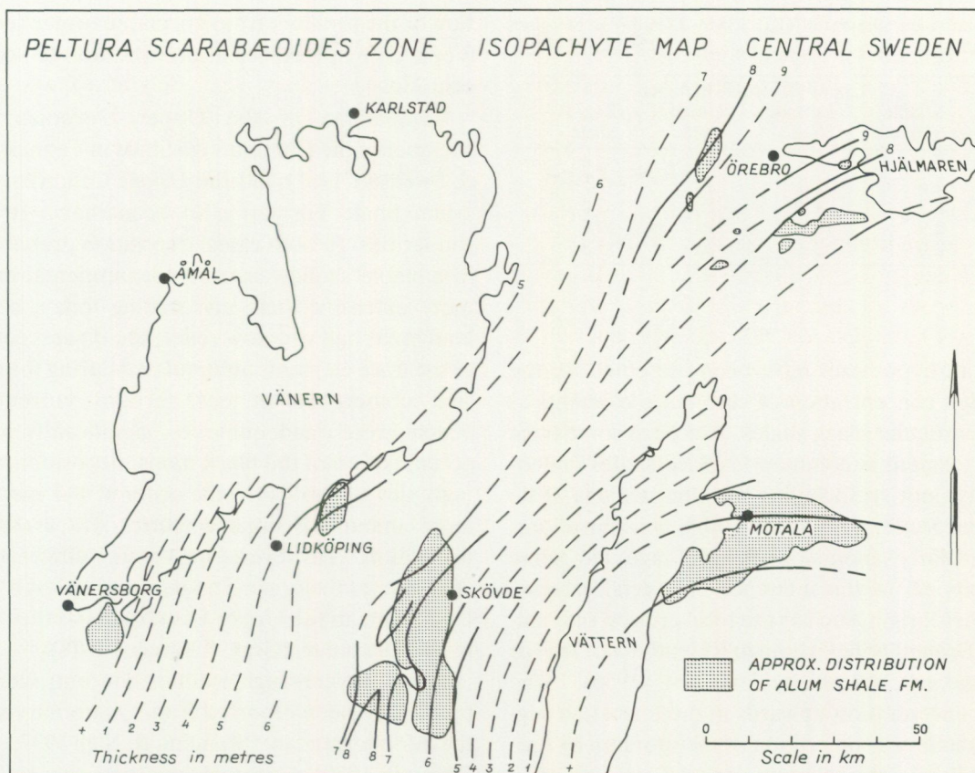
Fig. 23. Variations in thickness of the Pelatura scarabaeoides zone in the Närke, Östergötland and Västergötland outliers.
