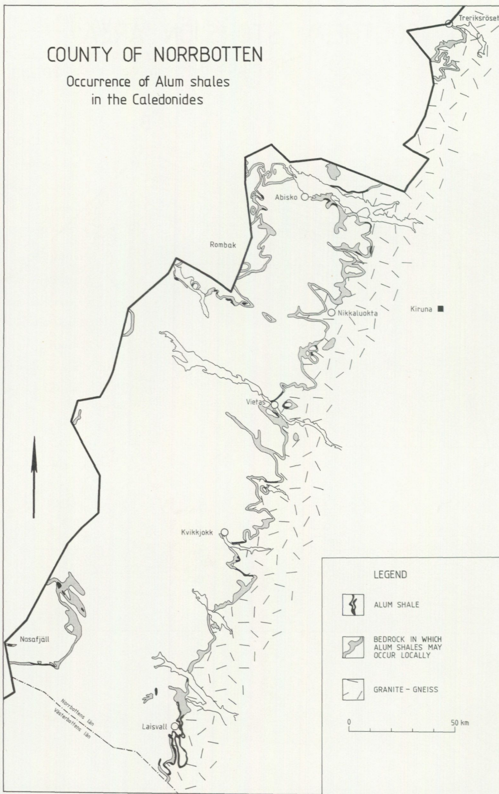
Fig. 20. Distribution of the alum shales in western Norrbotten County. The formation occurs sporadically in the autochthonous sedimentary rocks of the Caledonian Front, in the lower nappes and in the parautochthonous and lower allochthonous cover strata of the windows (based on a compilation for Radonutredningen 1979 by T. Thelander, Ds Jo 1979:9, Appendix 2:2).
