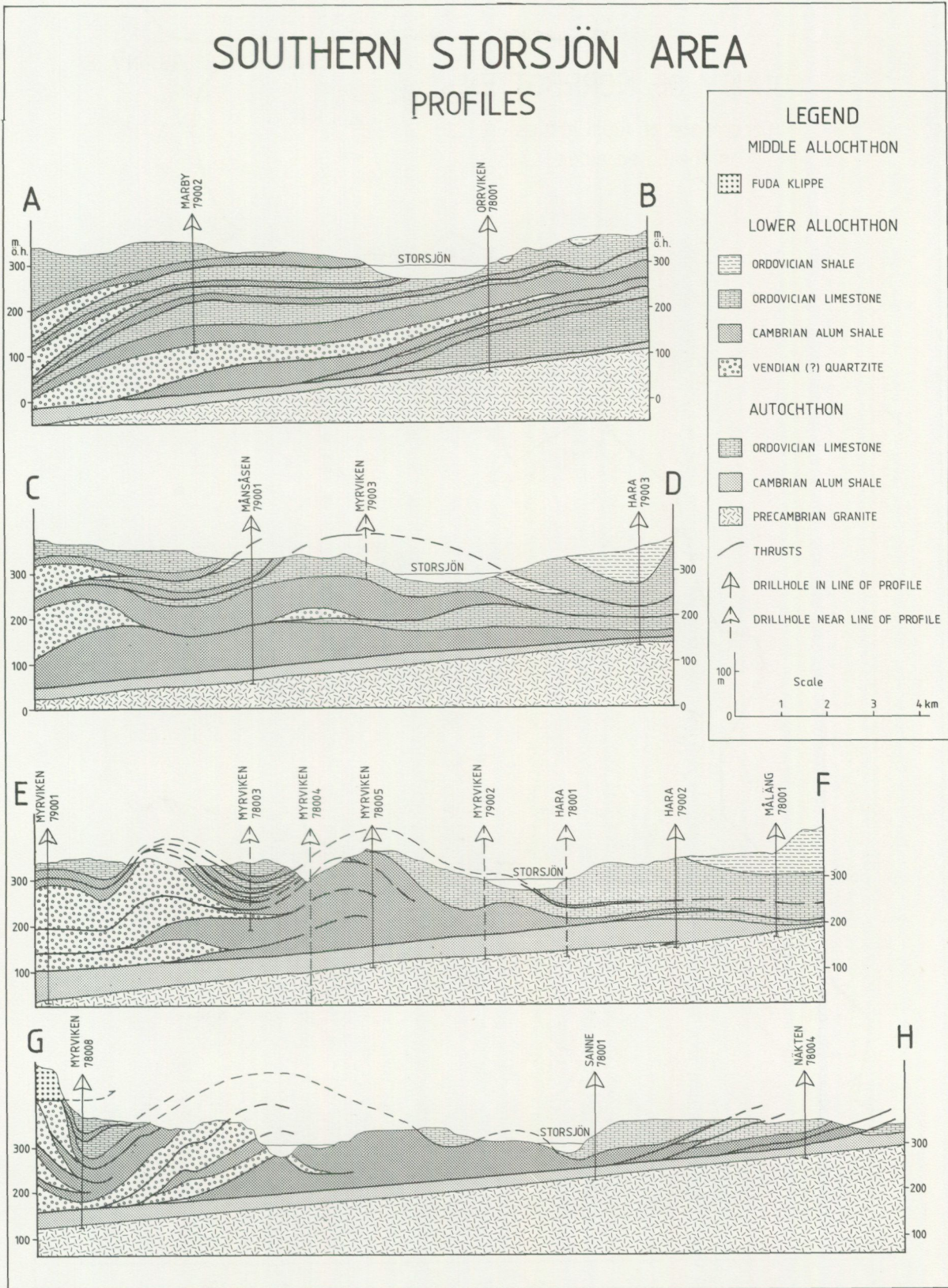
Fig. 19. Sections through the southern Storsjön area, Jämtland, (taken from Gee et al. 1982 unpublished report) illustrating the thick development of the alum shales where they are tectonically repeated in the core of the Myrviken Antiform. Note that the allochthonous cover of sedimentary rocks is thrust over a passive largely undisturbed autochthon of Cambrian shales (locally with Lower Ordovician limestones) and underlying Precambrian crystalline rocks.
