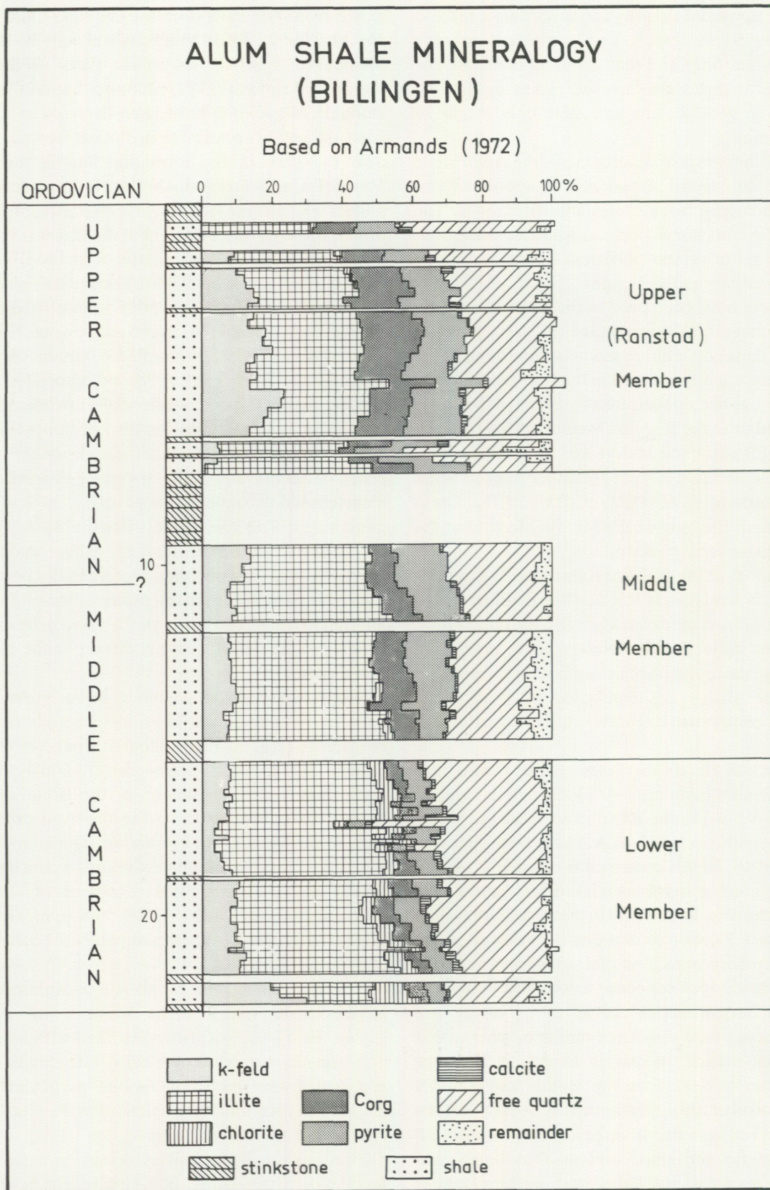
Fig. 6. Mineralogy of the Alum Shale Formation in the Billingen area based on Armands 1972. (Note that the boundary between the Middle and Upper Cambrian is not exactly defined).
