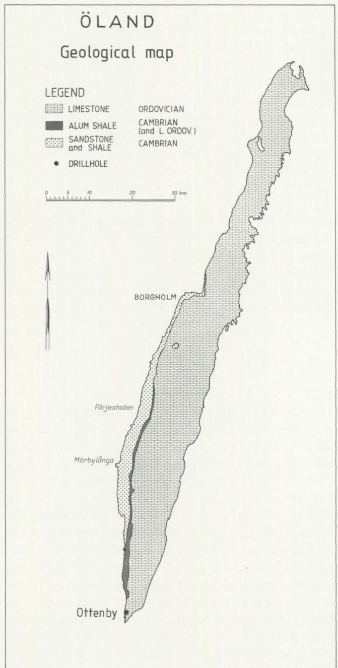
Fig. 16. Bedrock geology of the island of Öland (Hedström & Wiman 1906 and Dahlman 1977, unpublished report). In the northern part of the island the formation containing the alum shales is thin (<2 m) and dominated by stinkstones. It increases in thickness in southern Öland to a maximum of c. 23 m.
