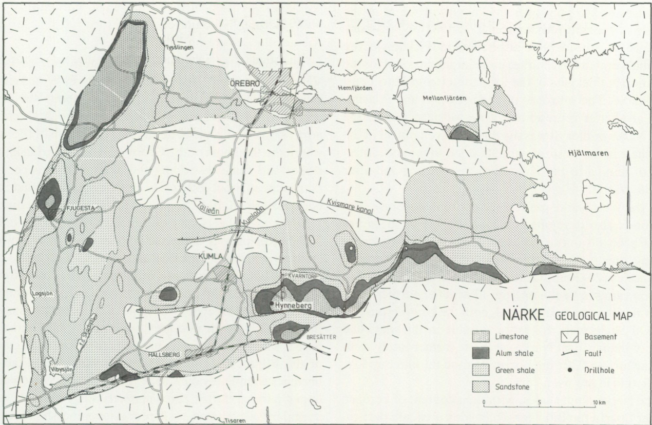
Fig. 12. Bedrock geology of the Närke area (from Eklund et al. 1961, Dahlman 1962, unpublished report, Lundegårdh & Fromm 1971 and Lundegårdh et al. 1972, 1973). The alum shales occur in two main outliers, referred to as East and West Närke.
