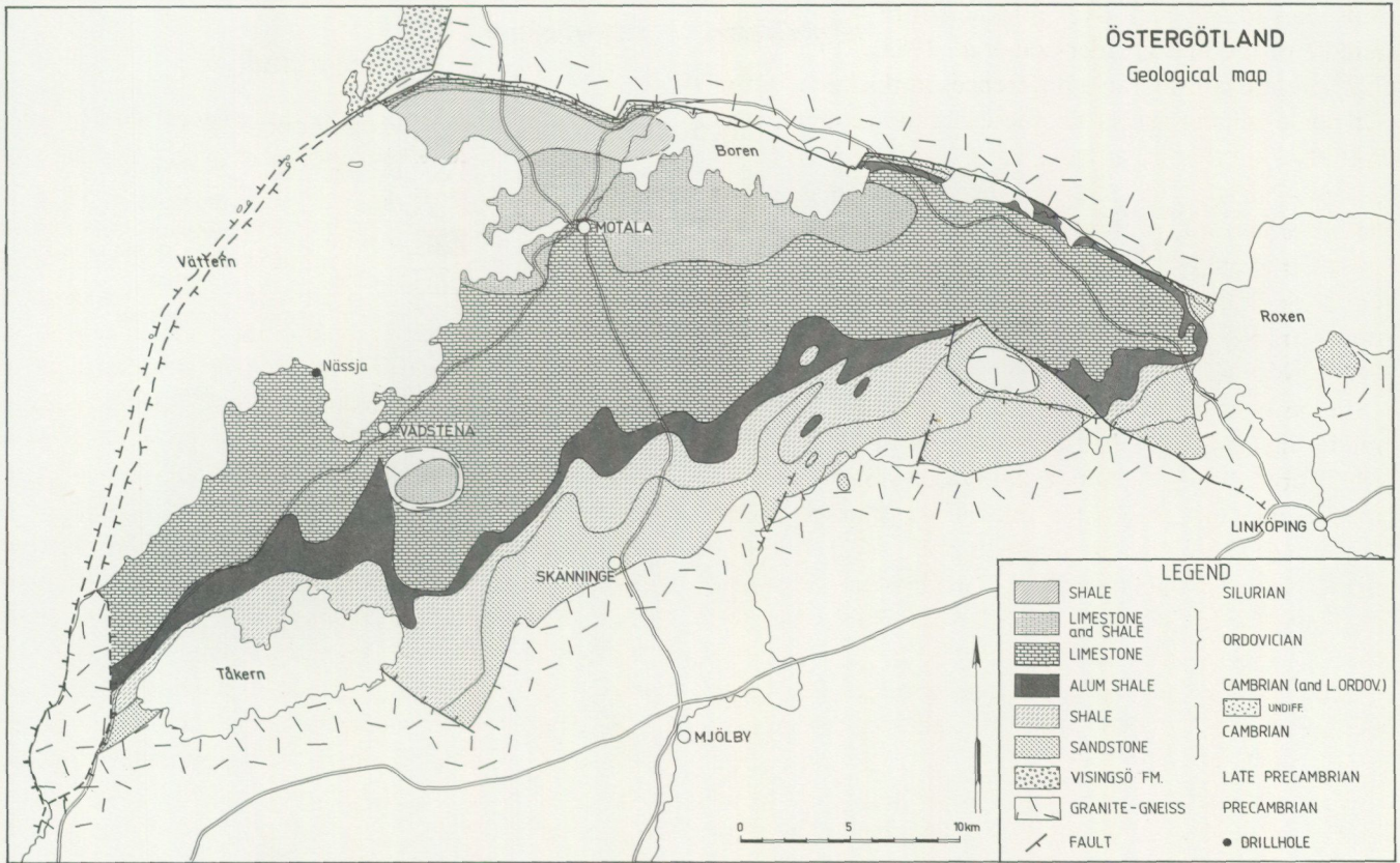
Fig. 14. Bedrock geology of the Östergötland outlier (from Thorslund 1944, Gorbatshev et al. 1976, Persson et al. 1981 and Wikman et al. 1980, 1982).
