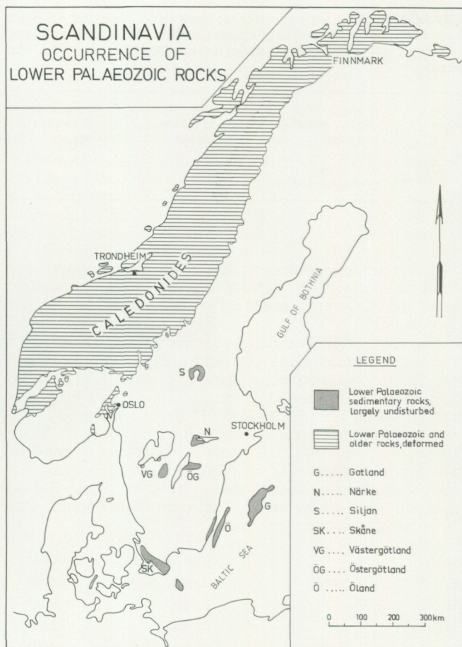
Fig. 1 Location of Lower Palaeozoic outliers and Caledonian orogen in Scandinavia.
