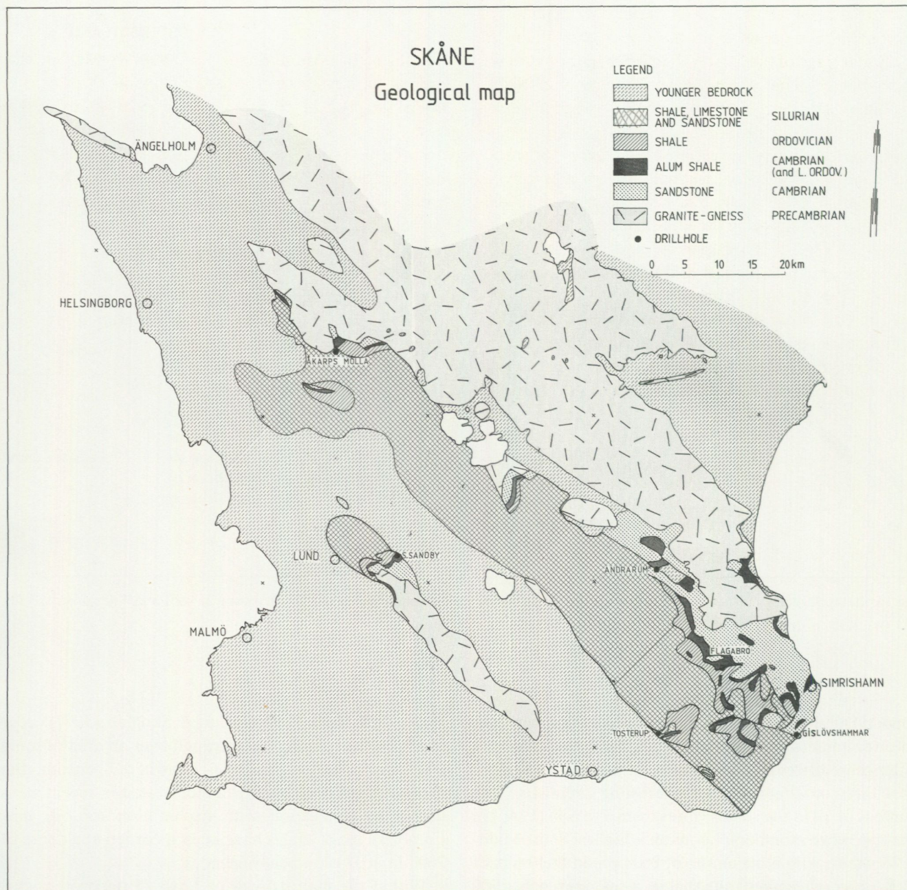
Fig. 15. Bedrock geology of Skåne. The distribution of the alum shales has been taken from Bergström & Shaikh (1980, 1982).
