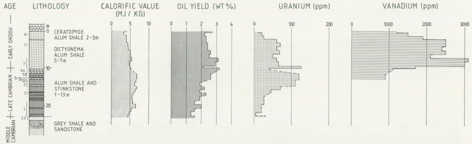
Fig. A6. The alum shales on Öland are illustrated by data from the Ottenby drillhole (Westergård 1944b). Analyses of uranium are taken from Dahlman & Eklund (1953, unpublished report). The thicknesses cited are representative of the southern part of the island, only.
