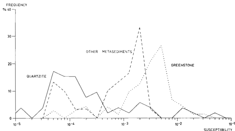
Fig. 11. In-situ susceptibility measurements on supracrustal rocks. Class width 0.2 decades.
