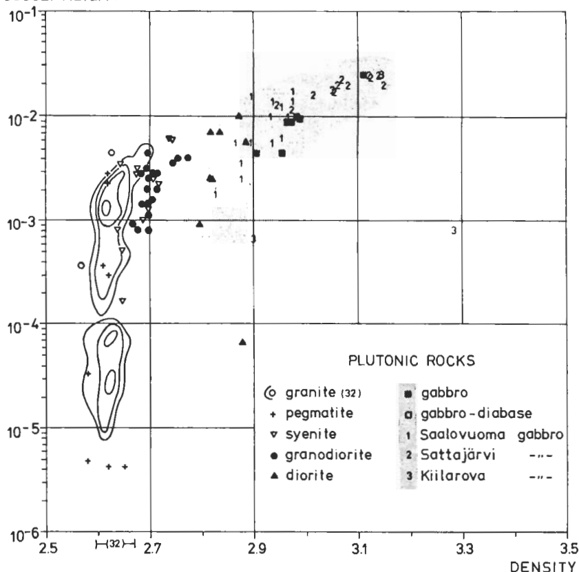
Fig. 18. Density — susceptibility diagram.
