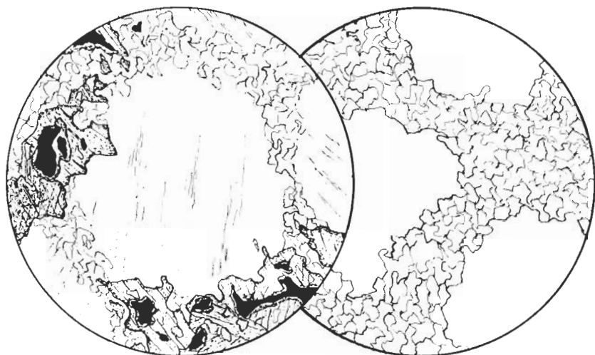
Fig. 22. (Normal light \times 18 .) Two examples of compartmented textures observed in perthite monzonites. Perthite cores displaying sutured boundaries are surrounded by a sutured fine-grained groundmass. Square 4i. "Cloisonnée"-textur i perthitmonzonit.
