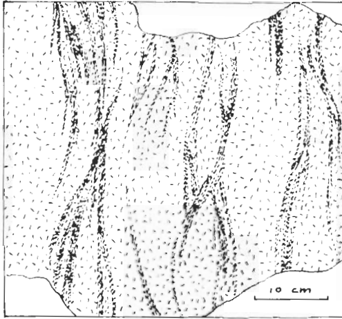
Fig. 14. Complex and irregular banding between a fine-grained pink porphyry (thin bands), and a pyroxene-bearing grey porphyry. Exposure north-west of Lau-lajavaara.
