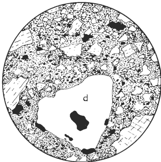
Fig. 15. (Normal light \times 20 .) Pyroclastic rock from a drill-hole in the Vivungi region. Mineral- (mainly augite) and rock-fragments are enclosed in a rather fine-grained chlorite-magnetite-feldspar groundmass. Muscovite and biotite are also present in the groundmass. D = diorite fragment. Pyroklastisk bergart ur borrhål från Vivungionrådet.
