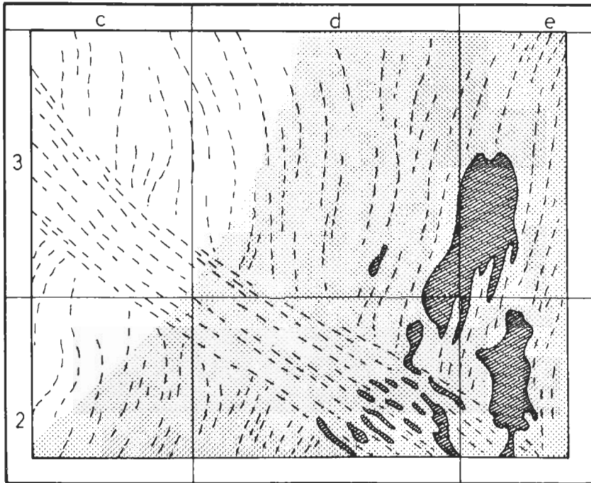
Fig. 40. Linear discontinuity of the strike of magnetic anomalies. The broken lines represent schematically the strike of the magnetic anomalies. The dark shadowed zones to the right are high magnetic anomalies (above 52 000 gammas) devoid of rock-exposures. The light grey represents an area where biotite schists and gneisses are rather well exposed. The non-shaded area is a Lina Granite massive. The normal magnetic trend, which is to north, is cut by a rather straight band in which the strike of the magnetic anomalies is to the north-west. Note the effect of this band on the high anomalies.
