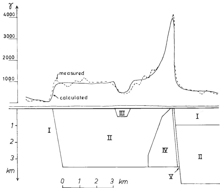
Fig. 74. 29L Lainio, aeromagnetic AT-profile P 110 over the Karijärvi anomaly. Susceptibilities of model-body: I = 0, II = 3,1, III = 0,8, IV = 8,1 and V = 12,8 \times 10^{-3} emu.
