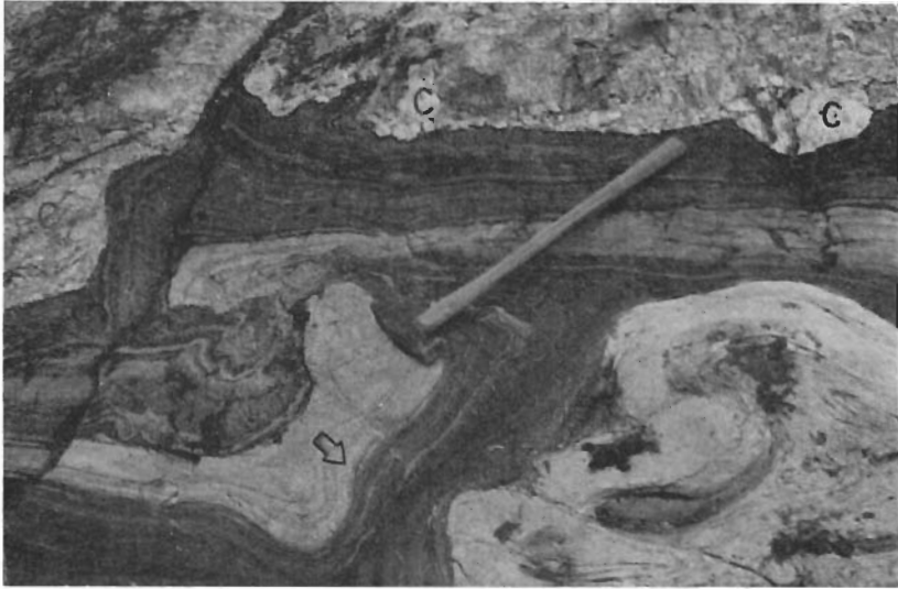
Fig. 10. Tightly folded meta-sediments in contact with a quartzitic conglomerate (C) at Paloleuska. Preserved cross-bedding in meta-sediments indicate a younging in the direction of the arrow. Veckade metasediment i kontakt med ett kvartsitbollförande konglomerat (C), Paloleuska. Bevarad strömsiktning i metasedimentet visar stratigrafiskt "uppåt" i pilens riktning.
