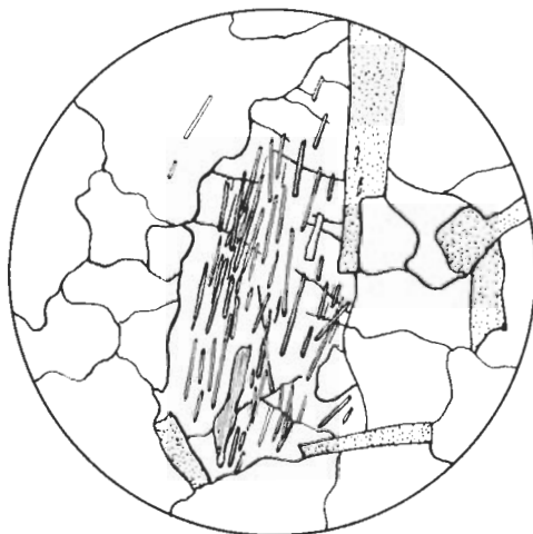
Fig. 11. (Normal light \times 45 .) Strongly recrystallized feldspathic quartzite at Palolenska. A fractured plagioclase contains a large quantity of more or less parallel minute silliminate needles, and a small muscovite flake. The shaded mineral is biotite.
