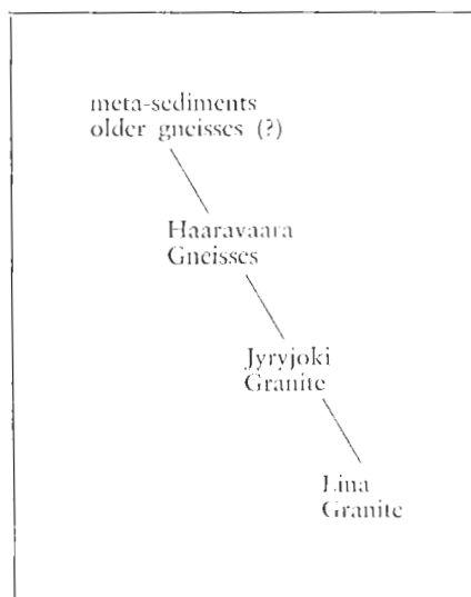
Fig. 16. Migmatitic series observed between different rock-types in the north-east of the map.
