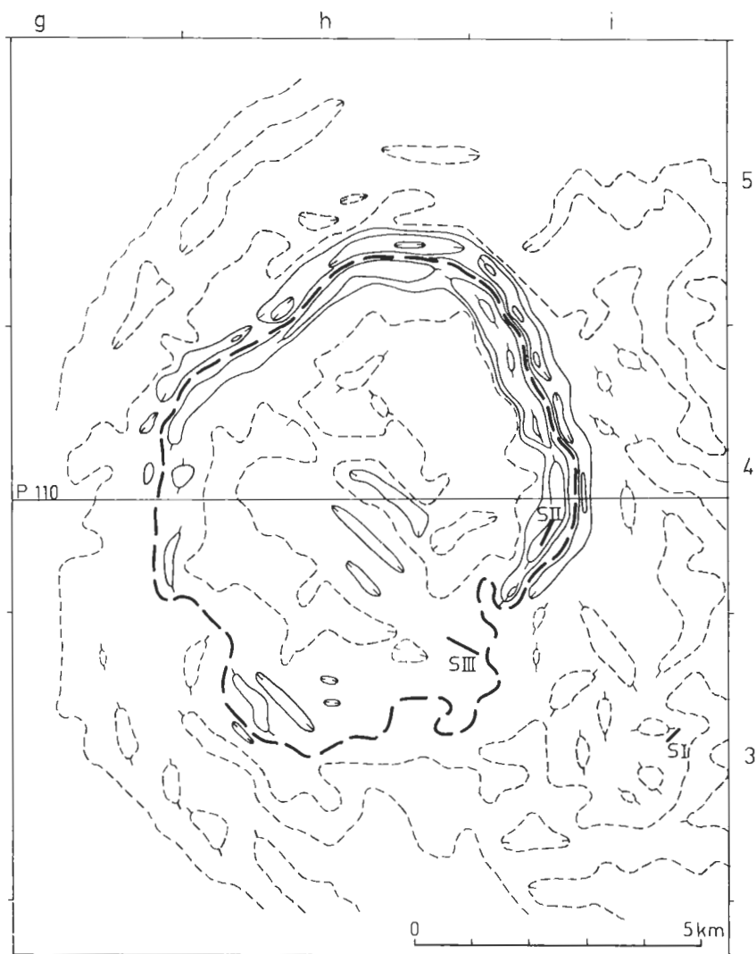
Fig. 73. Second vertical derivative ( \Delta T_{zz} ) of aeromagnetic total-intensity on the Karijärvi anomaly. Dashed lines denote \Delta T_{zz} - O . Heavily dashed zero-line gives the border of the anomalous body. SI-SIII are seismic profiles. Andra vertikala derivatan av aeromagnetiska totalintensiteten, Karijärvi-anomalien. SI-SIII seismiska profiler.
