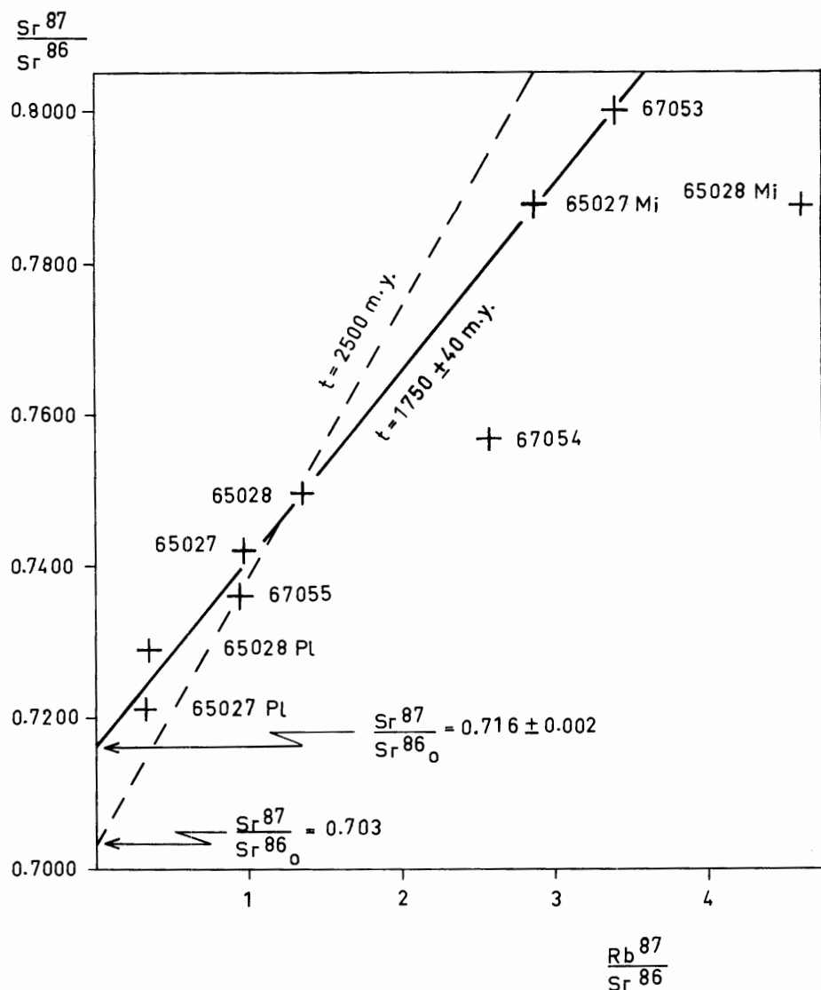
Fig. 2. Isochron diagram of whole rock and mineral samples from the Vuolosjärvi-Vakkosjärvi area, North Sweden.
