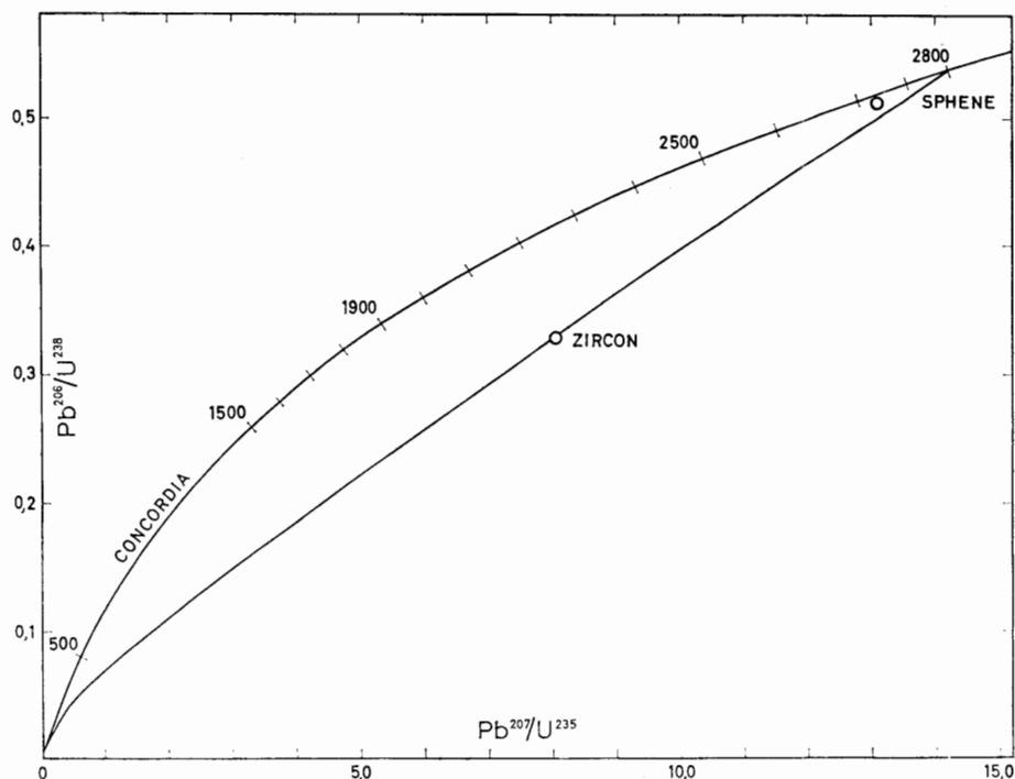
Fig. 3. Concordia-plot of zircon and sphene from sample 67055. Vuolonsjärvi-Vakkojärvi area, North Sweden. Analyst: Dr O. Kouvo, Geological Survey of Finland.
