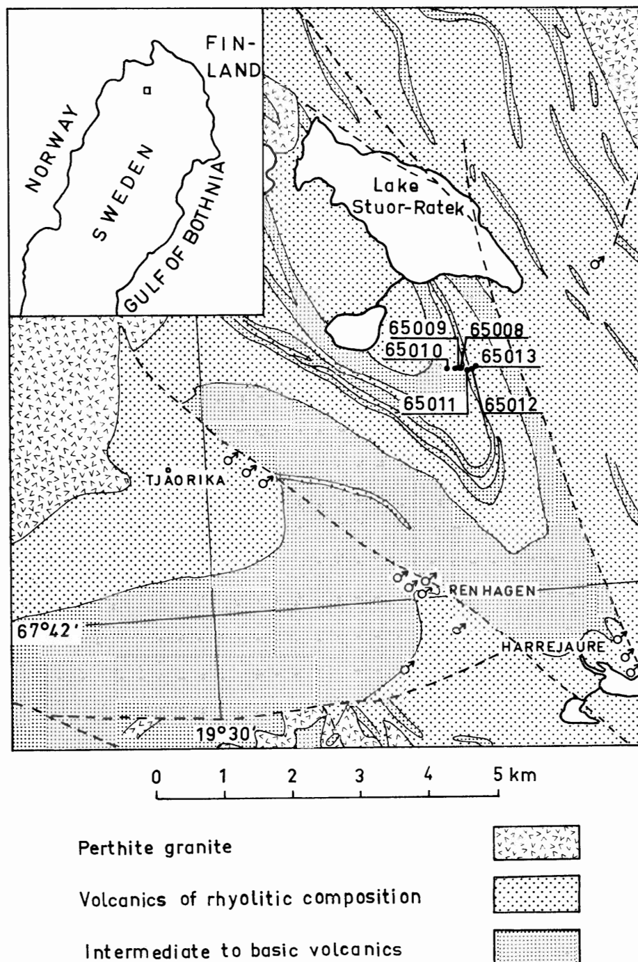
Fig. 13. Schematic geological map of the Kaska Tjåurek area, North Sweden, compiled from Offerberg (1967). Numbers refer to specimen localities.
