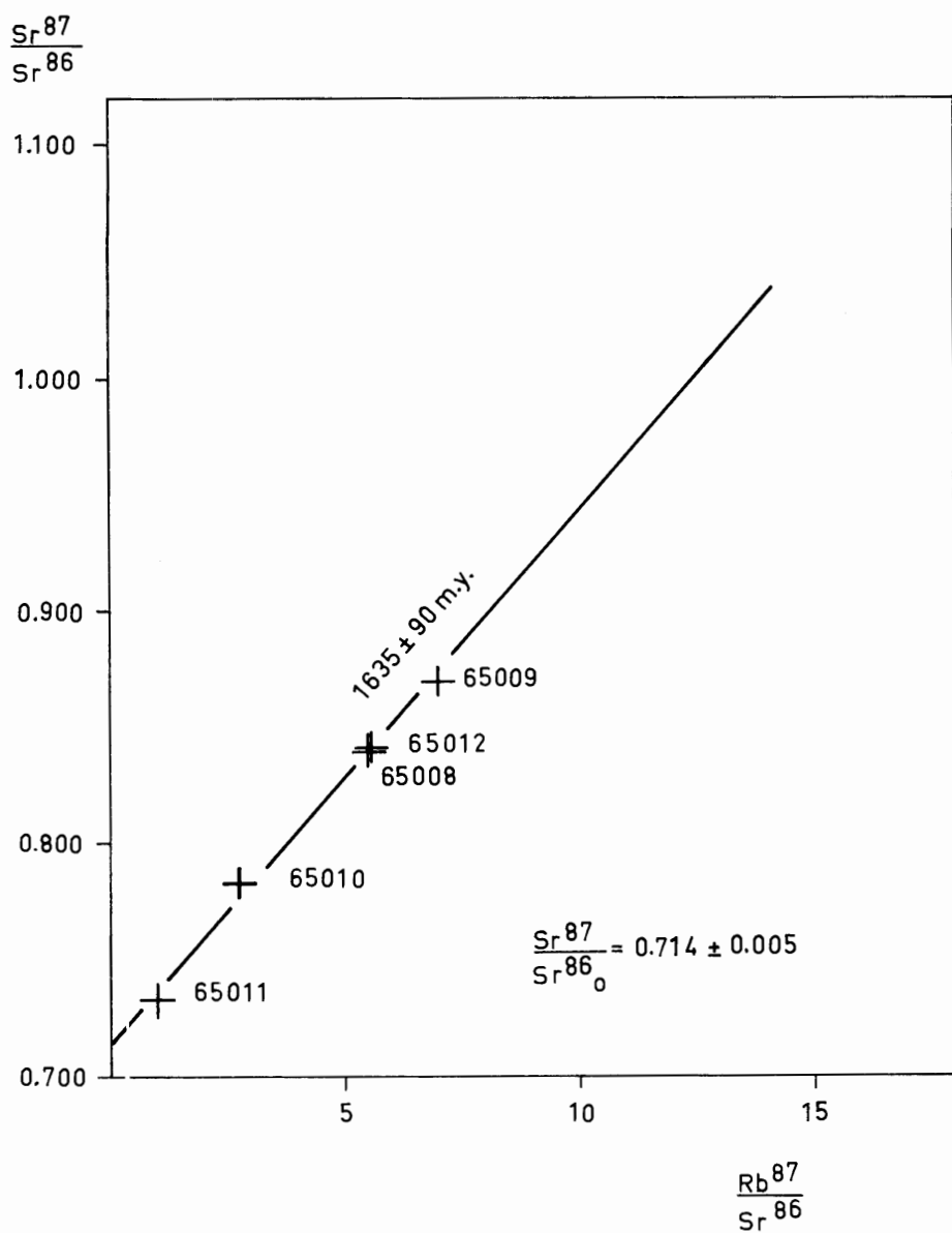
Fig. 14. Isochron diagram of whole rock samples from the Kaska Tjåurek area, North Sweden.
