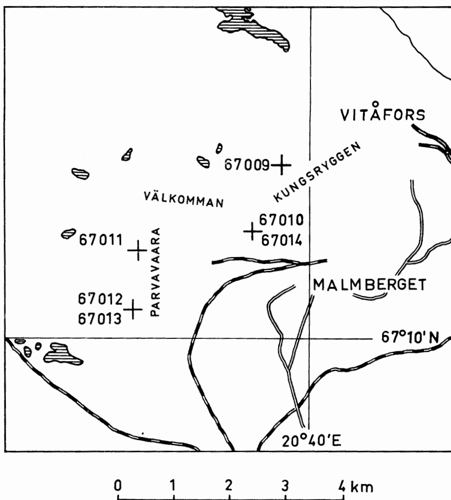
Fig. 9. Detailed map showing the location of the samples in the Malmberget area, North Sweden.
