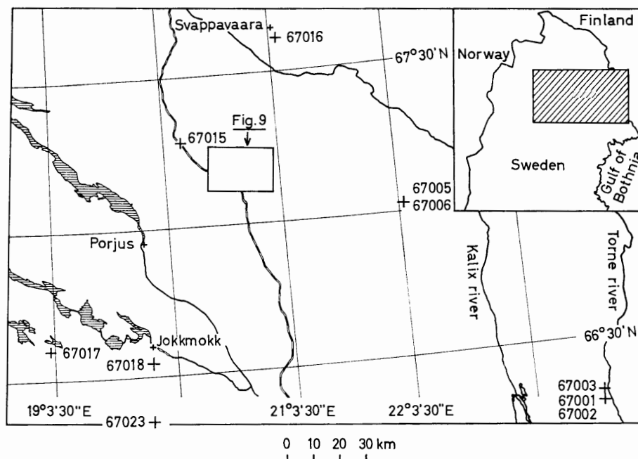
Fig. 8. Map showing the location of the Lina granite samples, North Sweden.
